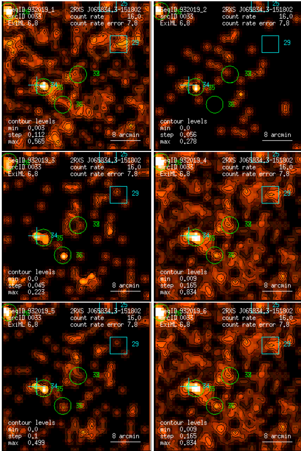
Figure 33: RASS 932019: detection 0033: band rate images, Gaussian filter: (1) PSPC channels 11 – 41, (2) 52 – 90, (3) 91 – 201, (4) 11 – 235, (5) 52 – 201, (6) 11 – 201. Broad band rates in counts/ks. Band rate contour levels in counts/ks/arcmin 2 .
