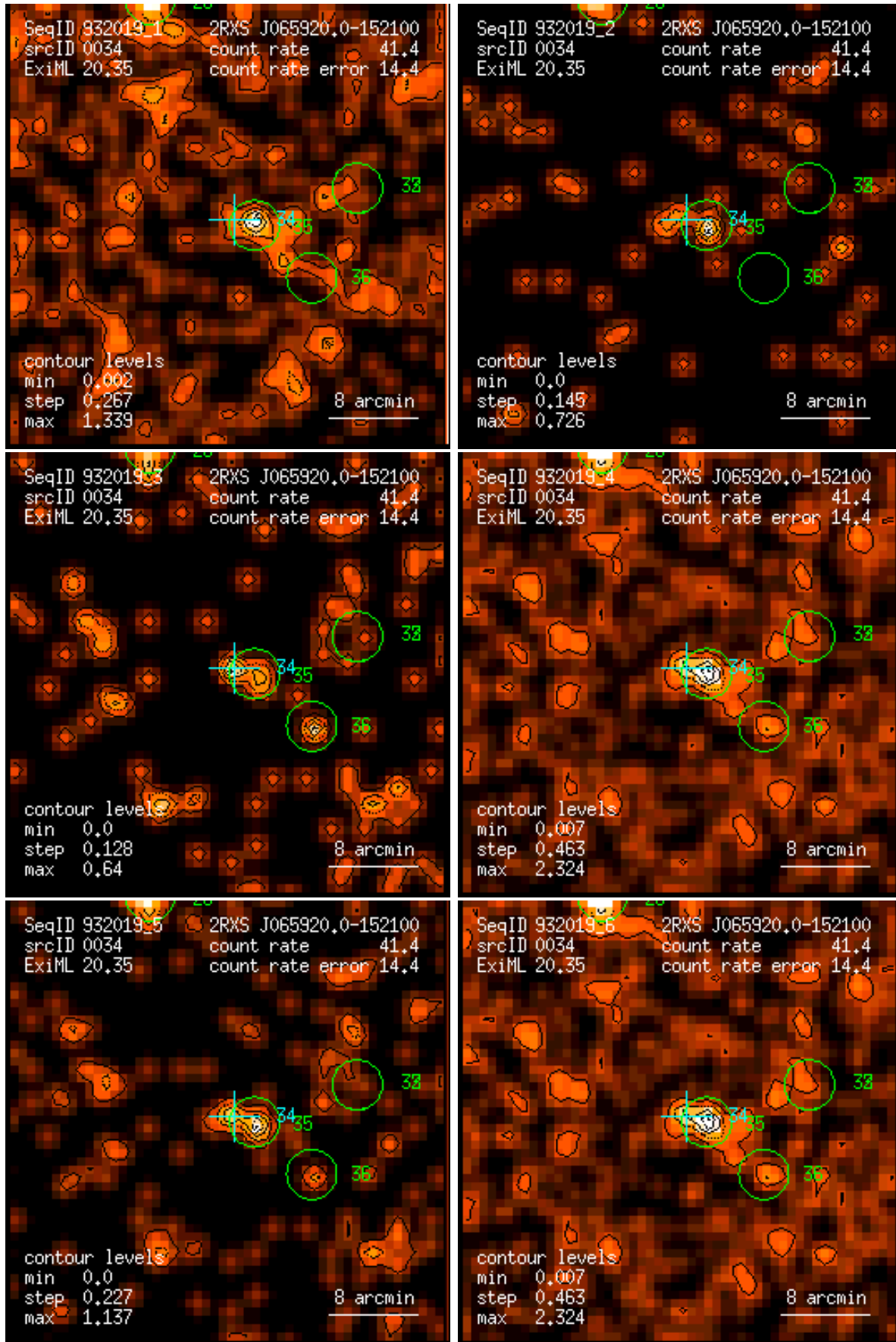
Figure 34: RASS 932019: detection 0034: band rate images, Gaussian filter: (1) PSPC channels 11 – 41, (2) 52 – 90, (3) 91 – 201, (4) 11 – 235, (5) 52 – 201, (6) 11 – 201. Broad band rates in counts/ks. Band rate contour levels in counts/ks/arcmin 2 .
