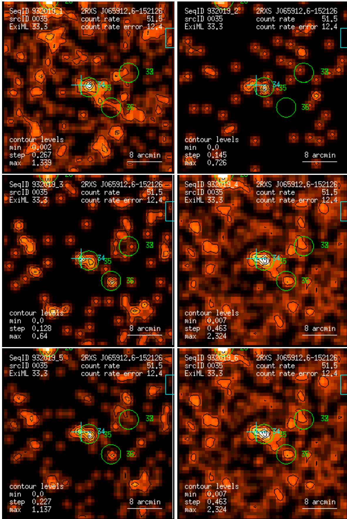
Figure 35: RASS 932019: detection 0035: band rate images, Gaussian filter: (1) PSPC channels 11 – 41, (2) 52 – 90, (3) 91 – 201, (4) 11 – 235, (5) 52 – 201, (6) 11 – 201. Broad band rates in counts/ks. Band rate contour levels in counts/ks/arcmin 2 .
