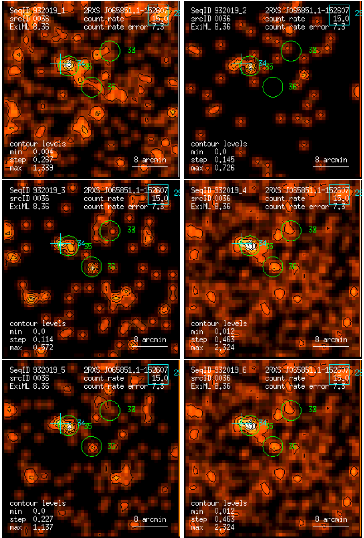
Figure 36: RASS 932019: detection 0036: band rate images, Gaussian filter: (1) PSPC channels 11 – 41, (2) 52 – 90, (3) 91 – 201, (4) 11 – 235, (5) 52 – 201, (6) 11 – 201. Broad band rates in counts/ks. Band rate contour levels in counts/ks/arcmin 2 .
