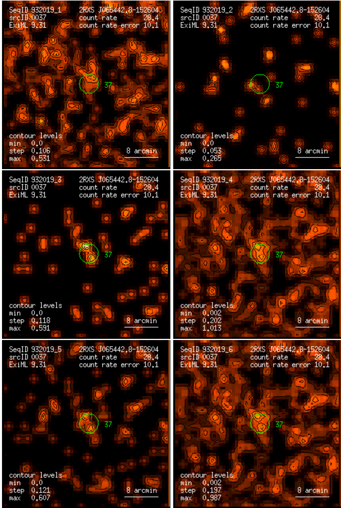
Figure 37: RASS 932019: detection 0037: band rate images, Gaussian filter: (1) PSPC channels 11 – 41, (2) 52 – 90, (3) 91 – 201, (4) 11 – 235, (5) 52 – 201, (6) 11 – 201. Broad band rates in counts/ks. Band rate contour levels in counts/ks/arcmin 2 .
