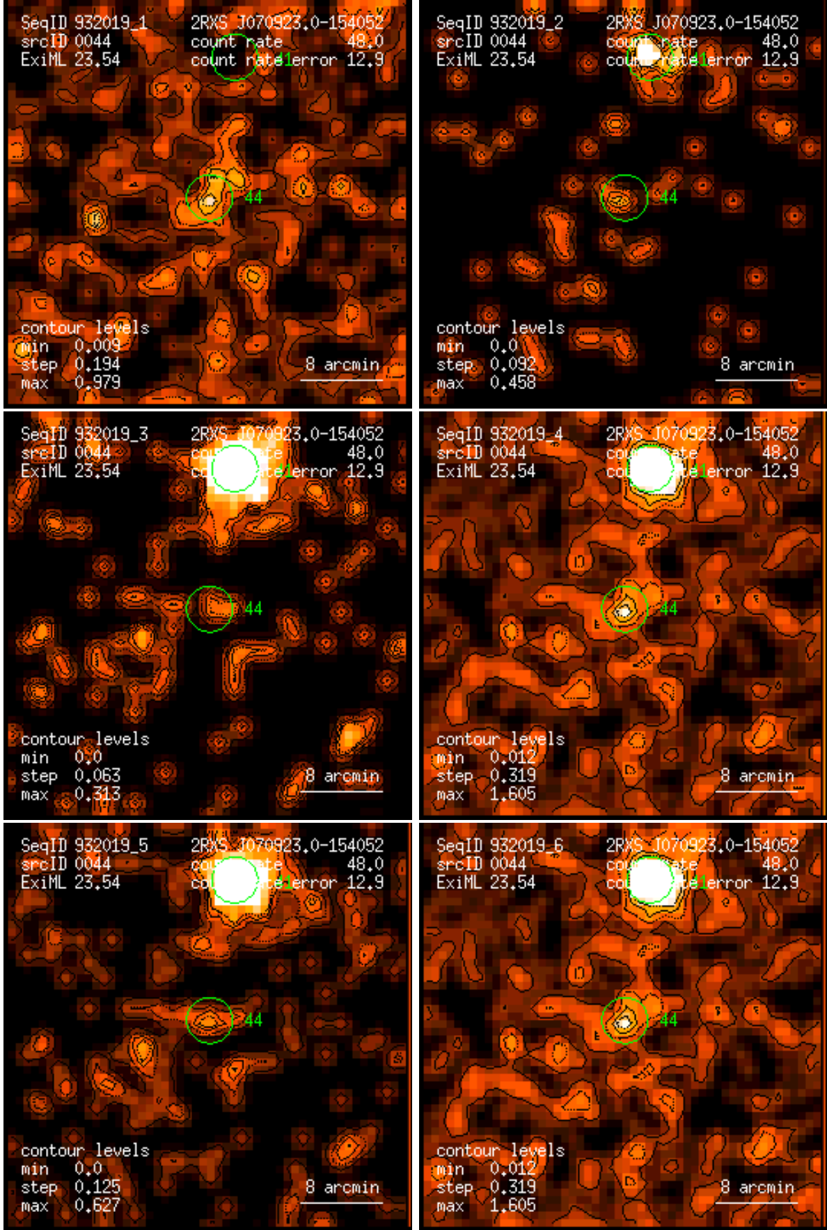
Figure 44: RASS 932019: detection 0044: band rate images, Gaussian filter: (1) PSPC channels 11 – 41, (2) 52 – 90, (3) 91 – 201, (4) 11 – 235, (5) 52 – 201, (6) 11 – 201. Broad band rates in counts/ks. Band rate contour levels in counts/ks/arcmin 2 .
