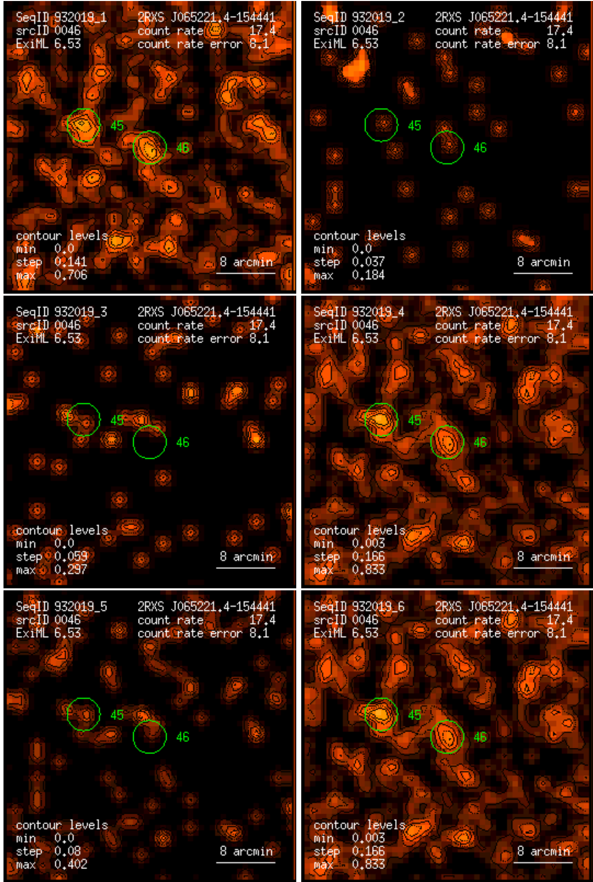
Figure 46: RASS 932019: detection 0046: band rate images, Gaussian filter: (1) PSPC channels 11 – 41, (2) 52 – 90, (3) 91 – 201, (4) 11 – 235, (5) 52 – 201, (6) 11 – 201. Broad band rates in counts/ks. Band rate contour levels in counts/ks/arcmin 2 .
