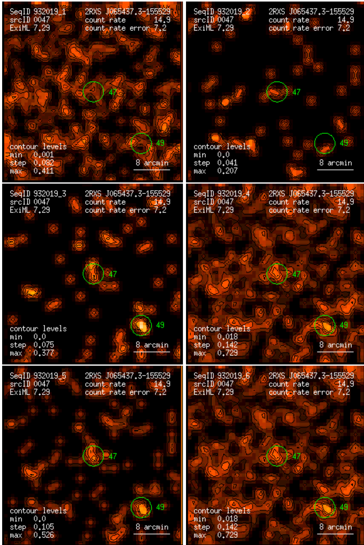
Figure 47: RASS 932019: detection 0047: band rate images, Gaussian filter: (1) PSPC channels 11 – 41, (2) 52 – 90, (3) 91 – 201, (4) 11 – 235, (5) 52 – 201, (6) 11 – 201. Broad band rates in counts/ks. Band rate contour levels in counts/ks/arcmin 2 .
