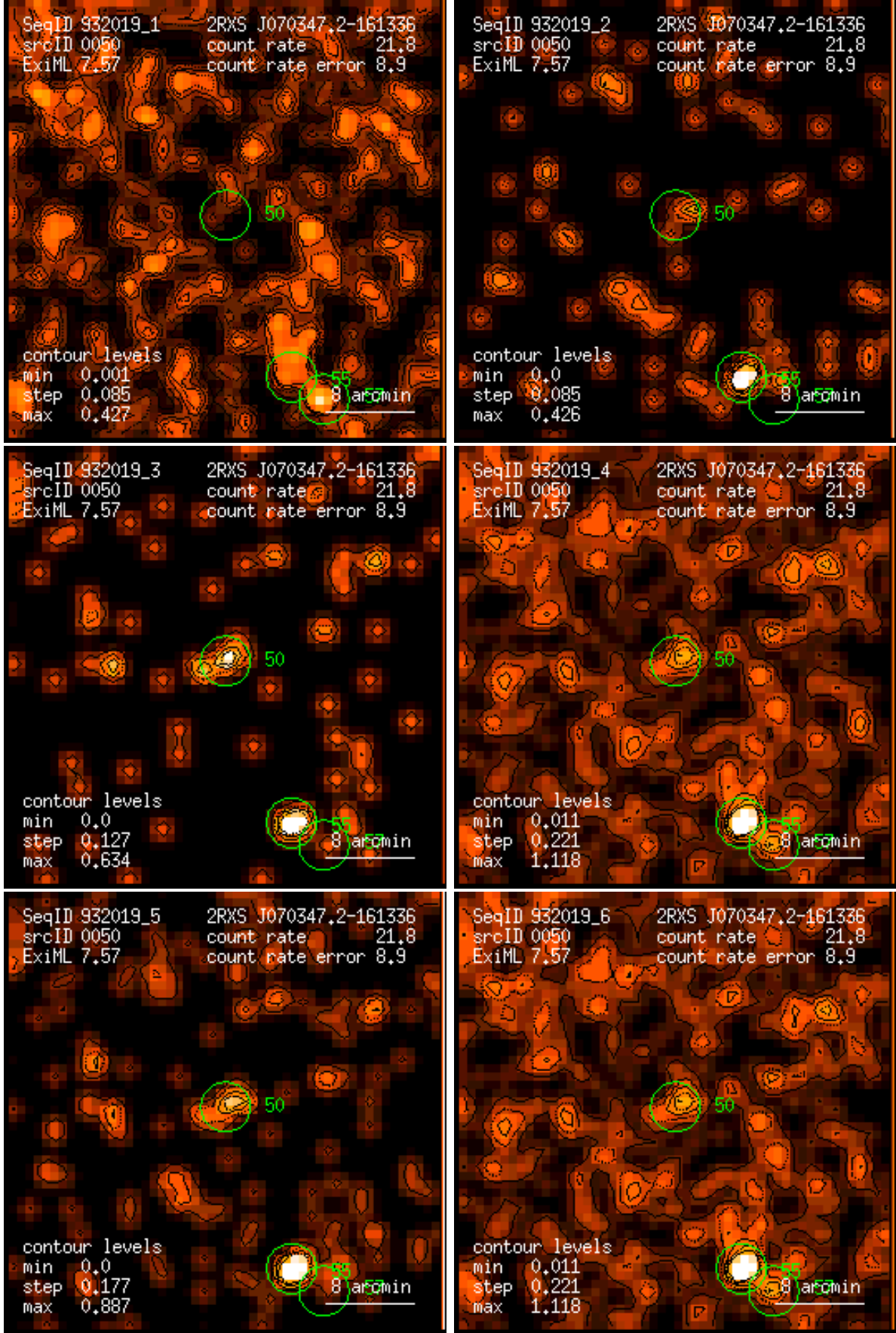
Figure 50: RASS 932019: detection 0050: band rate images, Gaussian filter: (1) PSPC channels 11 – 41, (2) 52 – 90, (3) 91 – 201, (4) 11 – 235, (5) 52 – 201, (6) 11 – 201. Broad band rates in counts/ks. Band rate contour levels in counts/ks/arcmin 2 .
