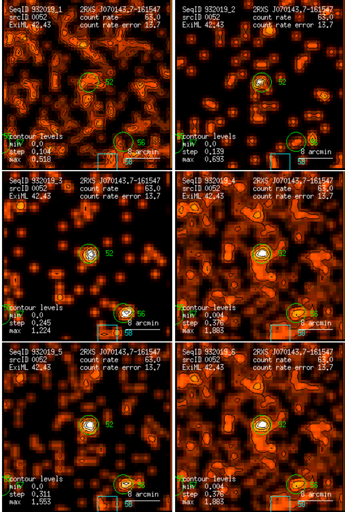
Figure 52: RASS 932019: detection 0052: band rate images, Gaussian filter: (1) PSPC channels 11 – 41, (2) 52 – 90, (3) 91 – 201, (4) 11 – 235, (5) 52 – 201, (6) 11 – 201. Broad band rates in counts/ks. Band rate contour levels in counts/ks/arcmin 2 .
