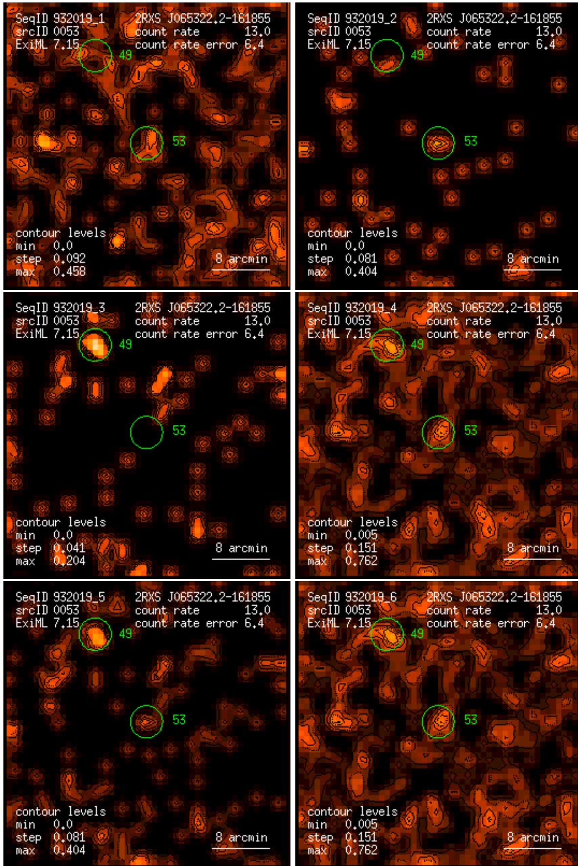
Figure 53: RASS 932019: detection 0053: band rate images, Gaussian filter: (1) PSPC channels 11 – 41, (2) 52 – 90, (3) 91 – 201, (4) 11 – 235, (5) 52 – 201, (6) 11 – 201. Broad band rates in counts/ks. Band rate contour levels in counts/ks/arcmin 2 .
