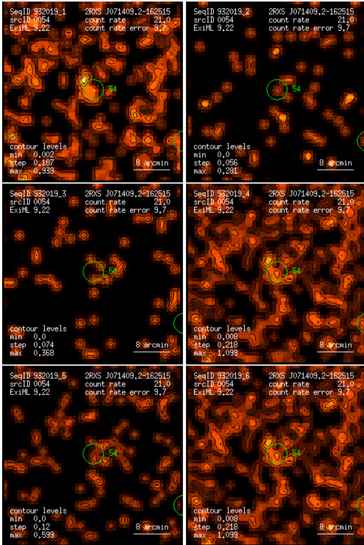
Figure 54: RASS 932019: detection 0054: band rate images, Gaussian filter: (1) PSPC channels 11 – 41, (2) 52 – 90, (3) 91 – 201, (4) 11 – 235, (5) 52 – 201, (6) 11 – 201. Broad band rates in counts/ks. Band rate contour levels in counts/ks/arcmin 2 .
