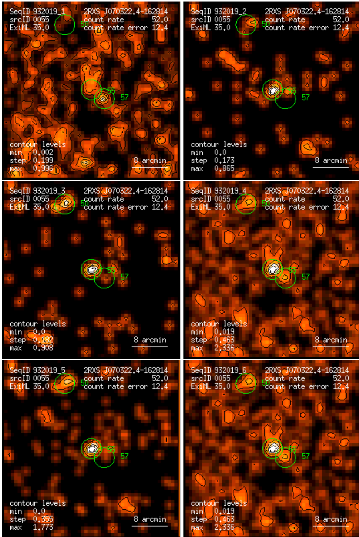
Figure 55: RASS 932019: detection 0055: band rate images, Gaussian filter: (1) PSPC channels 11 – 41, (2) 52 – 90, (3) 91 – 201, (4) 11 – 235, (5) 52 – 201, (6) 11 – 201. Broad band rates in counts/ks. Band rate contour levels in counts/ks/arcmin 2 .
