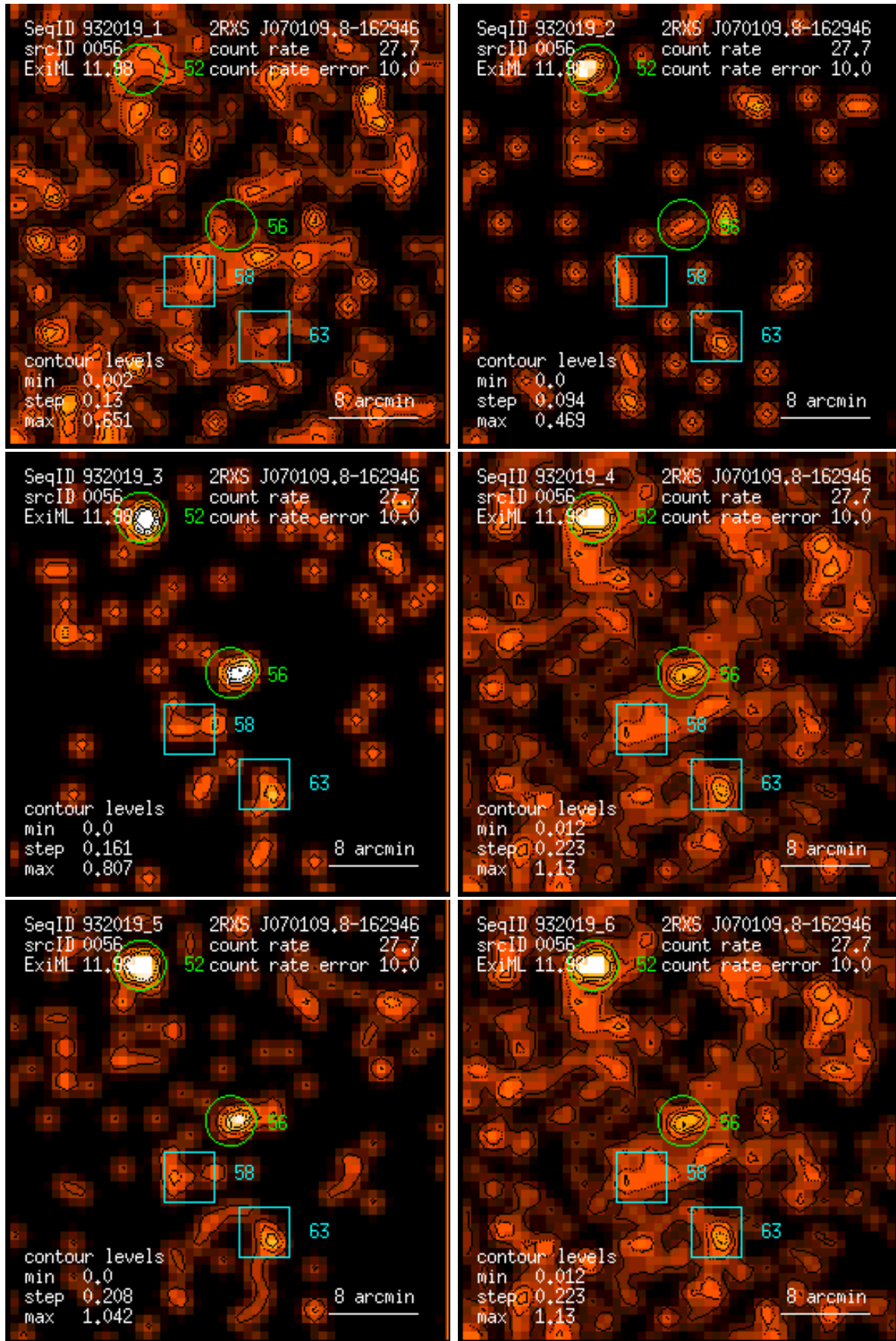
Figure 56: RASS 932019: detection 0056: band rate images, Gaussian filter: (1) PSPC channels 11 – 41, (2) 52 – 90, (3) 91 – 201, (4) 11 – 235, (5) 52 – 201, (6) 11 – 201. Broad band rates in counts/ks. Band rate contour levels in counts/ks/arcmin 2 .
