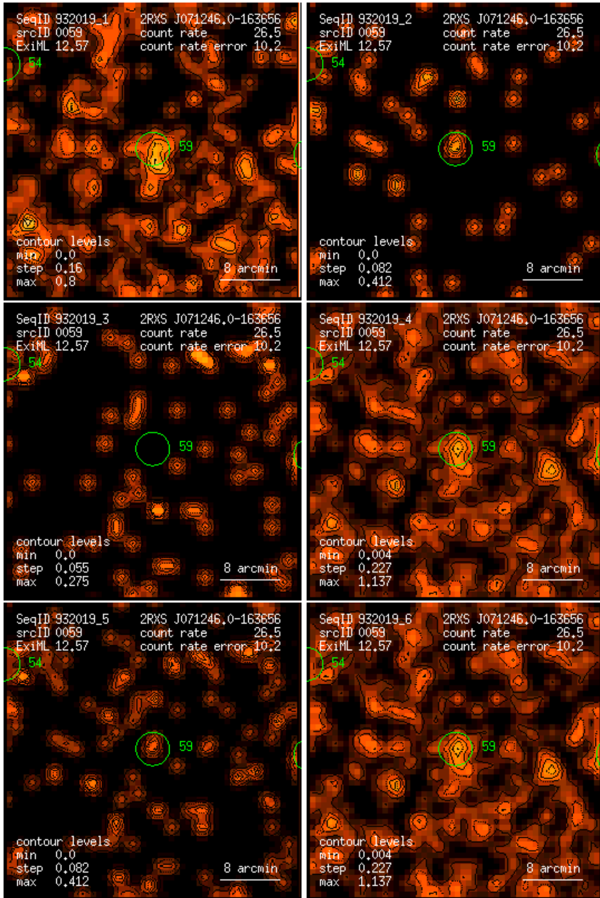
Figure 59: RASS 932019: detection 0059: band rate images, Gaussian filter: (1) PSPC channels 11 – 41, (2) 52 – 90, (3) 91 – 201, (4) 11 – 235, (5) 52 – 201, (6) 11 – 201. Broad band rates in counts/ks. Band rate contour levels in counts/ks/arcmin 2 .
