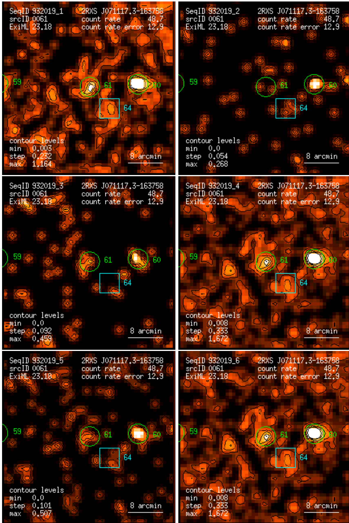
Figure 61: RASS 932019: detection 0061: band rate images, Gaussian filter: (1) PSPC channels 11 – 41, (2) 52 – 90, (3) 91 – 201, (4) 11 – 235, (5) 52 – 201, (6) 11 – 201. Broad band rates in counts/ks. Band rate contour levels in counts/ks/arcmin 2 .
