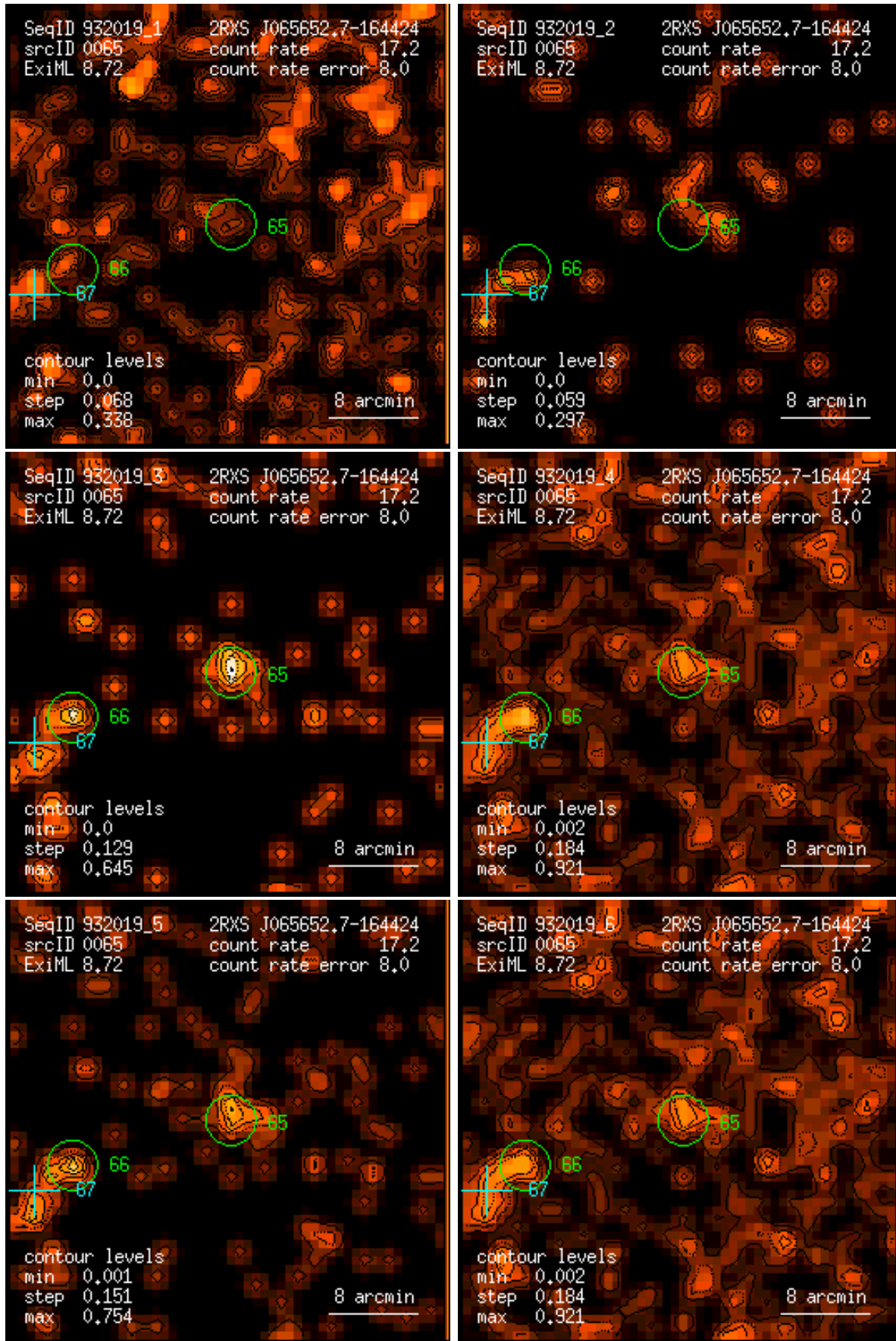
Figure 65: RASS 932019: detection 0065: band rate images, Gaussian filter: (1) PSPC channels 11 – 41, (2) 52 – 90, (3) 91 – 201, (4) 11 – 235, (5) 52 – 201, (6) 11 – 201. Broad band rates in counts/ks. Band rate contour levels in counts/ks/arcmin 2 .
