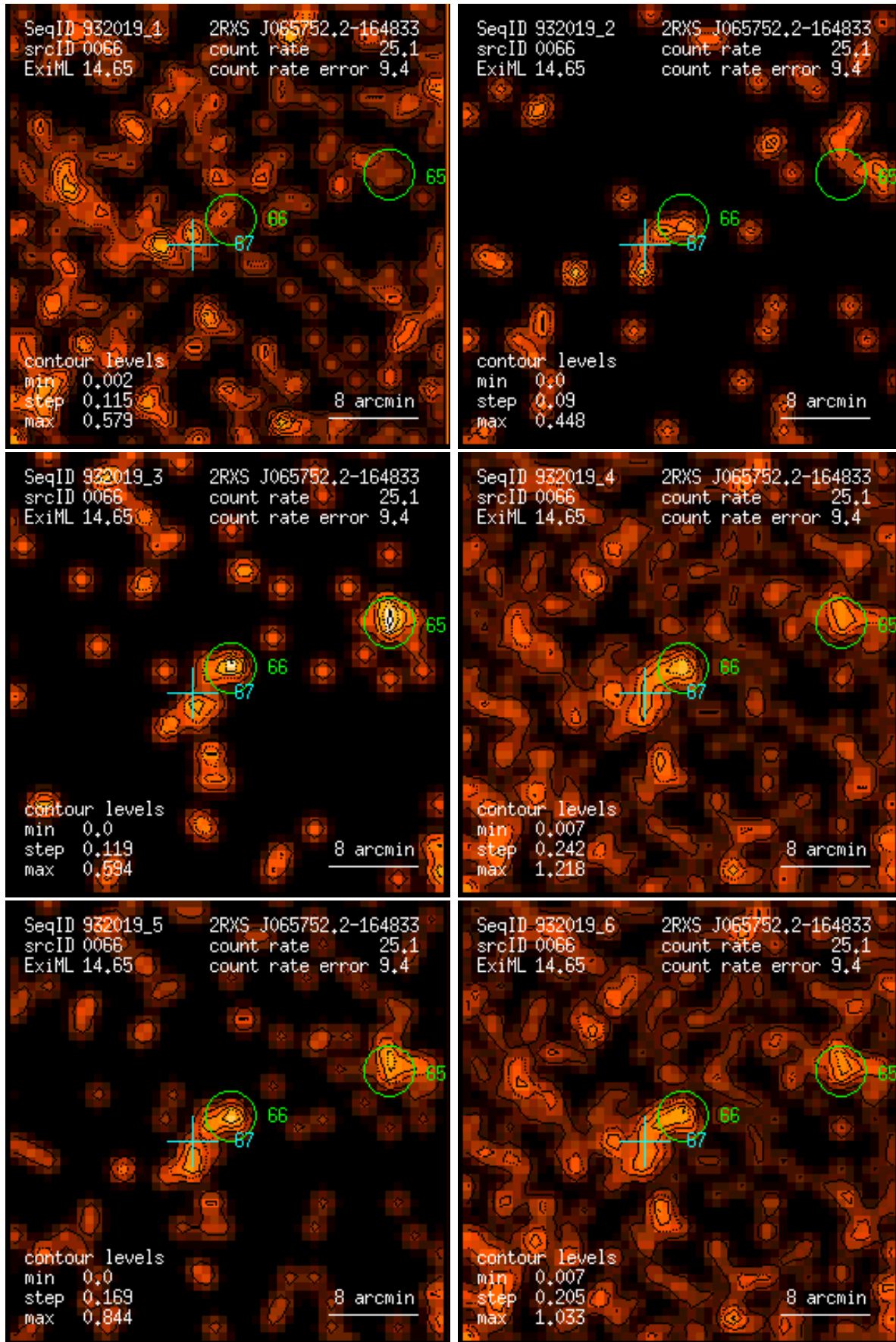
Figure 66: RASS 932019: detection 0066: band rate images, Gaussian filter: (1) PSPC channels 11 – 41, (2) 52 – 90, (3) 91 – 201, (4) 11 – 235, (5) 52 – 201, (6) 11 – 201. Broad band rates in counts/ks. Band rate contour levels in counts/ks/arcmin 2 .
