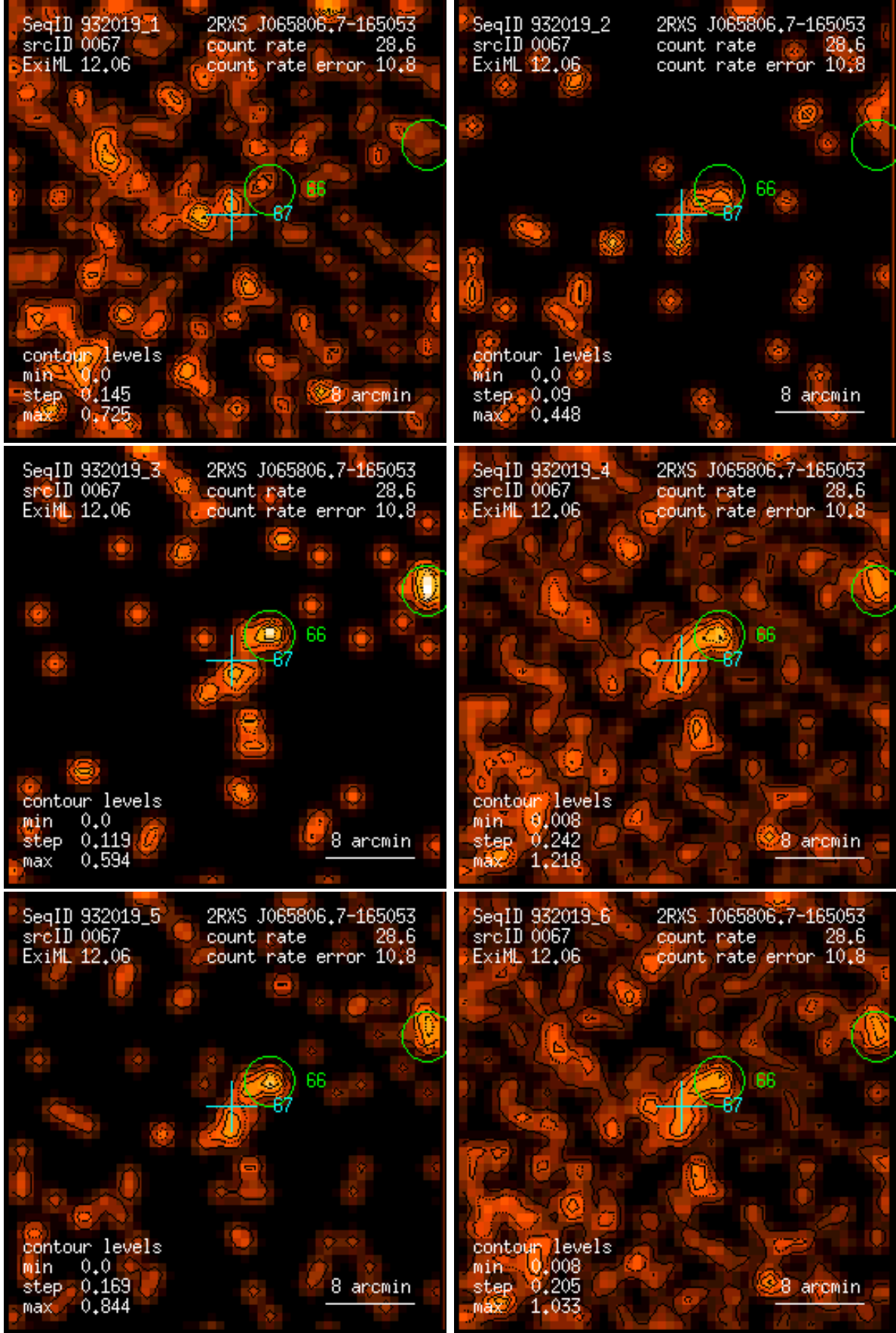
Figure 67: RASS 932019: detection 0067: band rate images, Gaussian filter: (1) PSPC channels 11 – 41, (2) 52 – 90, (3) 91 – 201, (4) 11 – 235, (5) 52 – 201, (6) 11 – 201. Broad band rates in counts/ks. Band rate contour levels in counts/ks/arcmin 2 .
