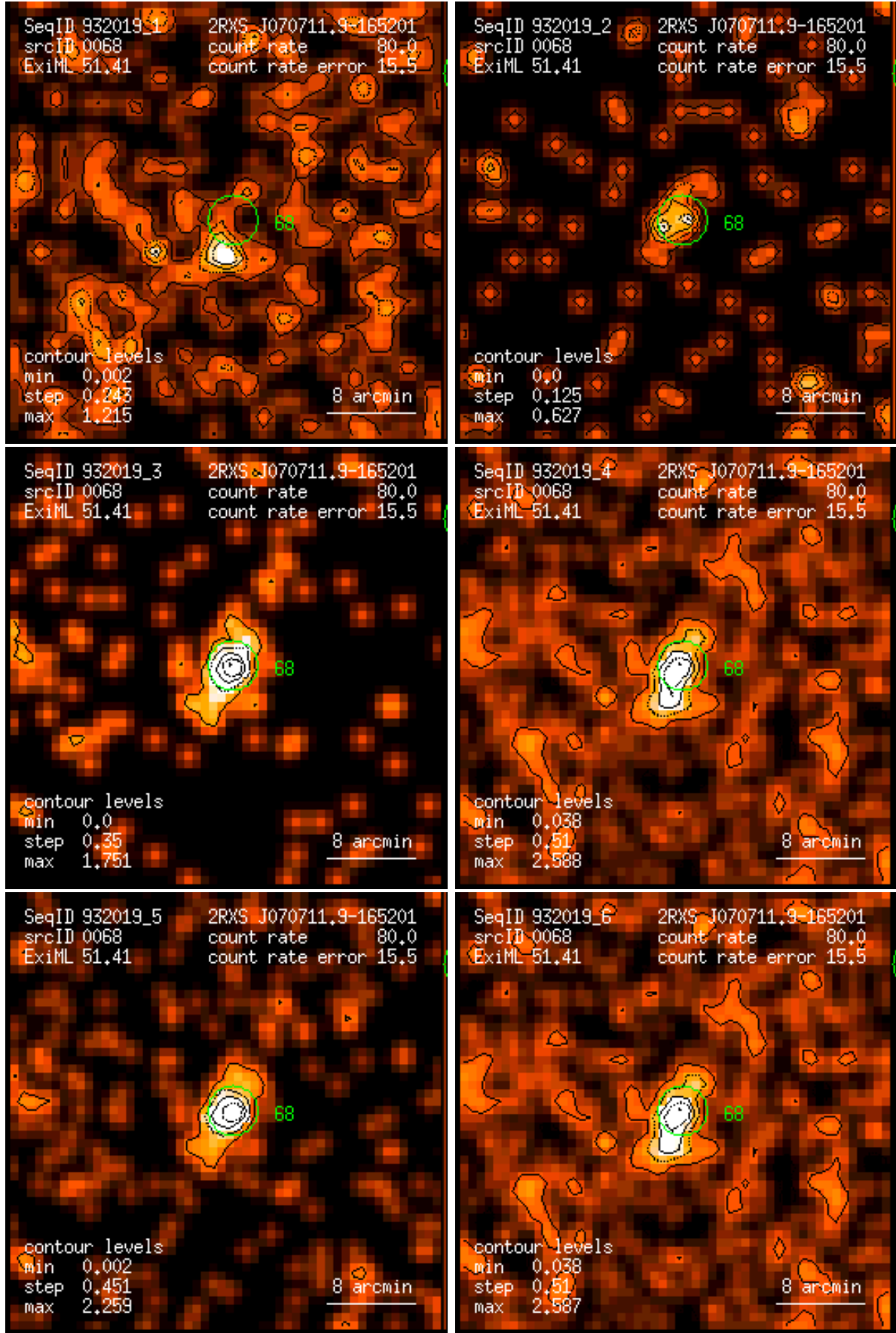
Figure 68: RASS 932019: detection 0068: band rate images, Gaussian filter: (1) PSPC channels 11 – 41, (2) 52 – 90, (3) 91 – 201, (4) 11 – 235, (5) 52 – 201, (6) 11 – 201. Broad band rates in counts/ks. Band rate contour levels in counts/ks/arcmin 2 .
