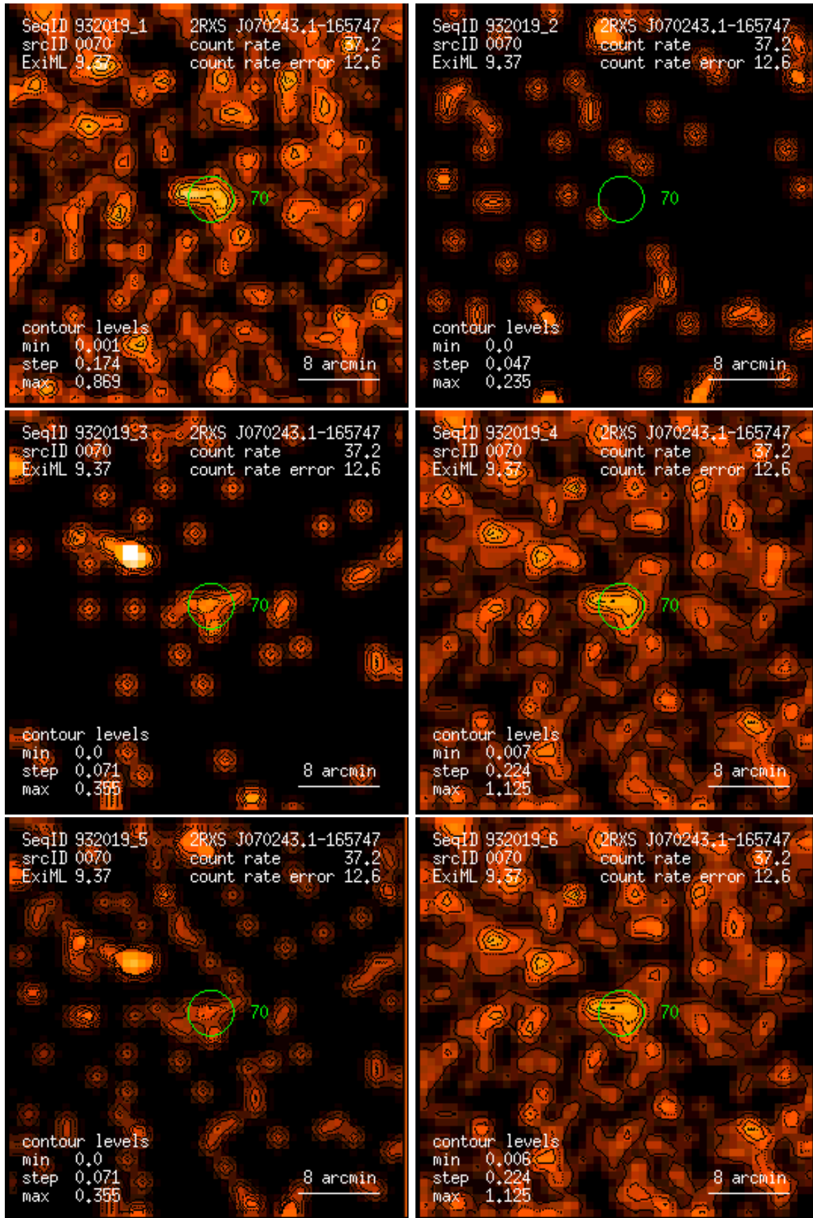
Figure 70: RASS 932019: detection 0070: band rate images, Gaussian filter: (1) PSPC channels 11 – 41, (2) 52 – 90, (3) 91 – 201, (4) 11 – 235, (5) 52 – 201, (6) 11 – 201. Broad band rates in counts/ks. Band rate contour levels in counts/ks/arcmin 2 .
