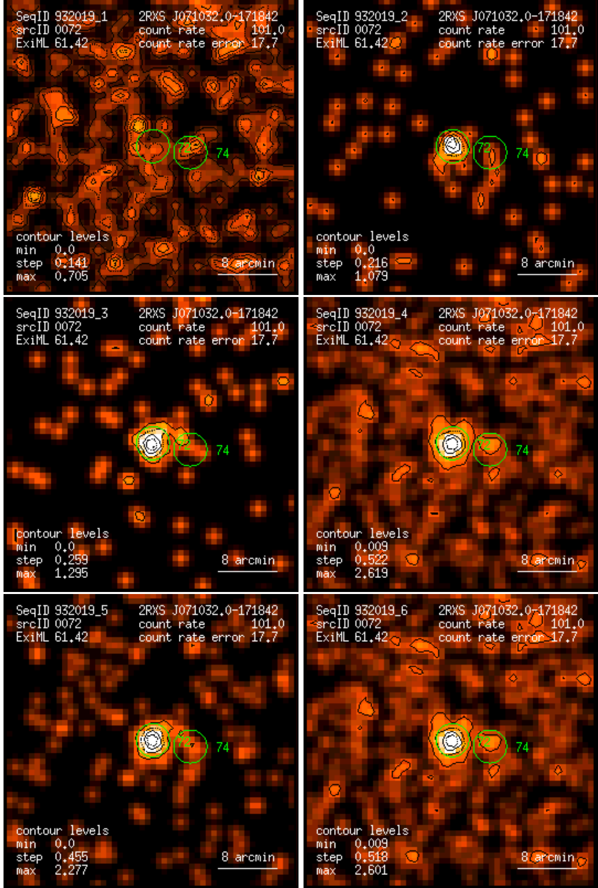
Figure 72: RASS 932019: detection 0072: band rate images, Gaussian filter: (1) PSPC channels 11 – 41, (2) 52 – 90, (3) 91 – 201, (4) 11 – 235, (5) 52 – 201, (6) 11 – 201. Broad band rates in counts/ks. Band rate contour levels in counts/ks/arcmin 2 .
