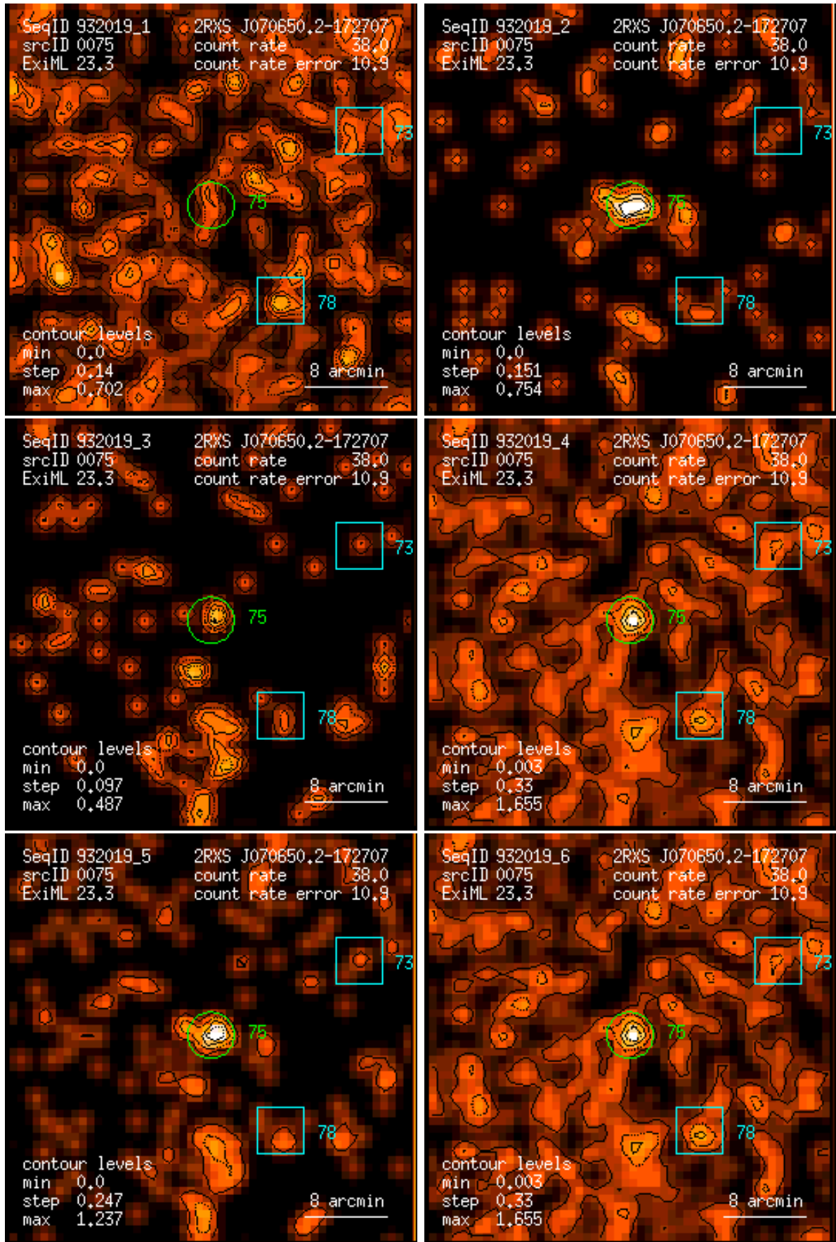
Figure 75: RASS 932019: detection 0075: band rate images, Gaussian filter: (1) PSPC channels 11 – 41, (2) 52 – 90, (3) 91 – 201, (4) 11 – 235, (5) 52 – 201, (6) 11 – 201. Broad band rates in counts/ks. Band rate contour levels in counts/ks/arcmin 2 .
