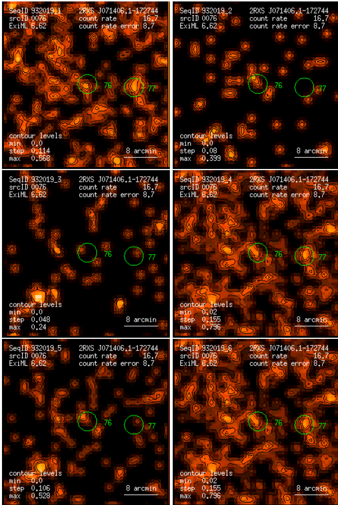
Figure 76: RASS 932019: detection 0076: band rate images, Gaussian filter: (1) PSPC channels 11 – 41, (2) 52 – 90, (3) 91 – 201, (4) 11 – 235, (5) 52 – 201, (6) 11 – 201. Broad band rates in counts/ks. Band rate contour levels in counts/ks/arcmin 2 .
