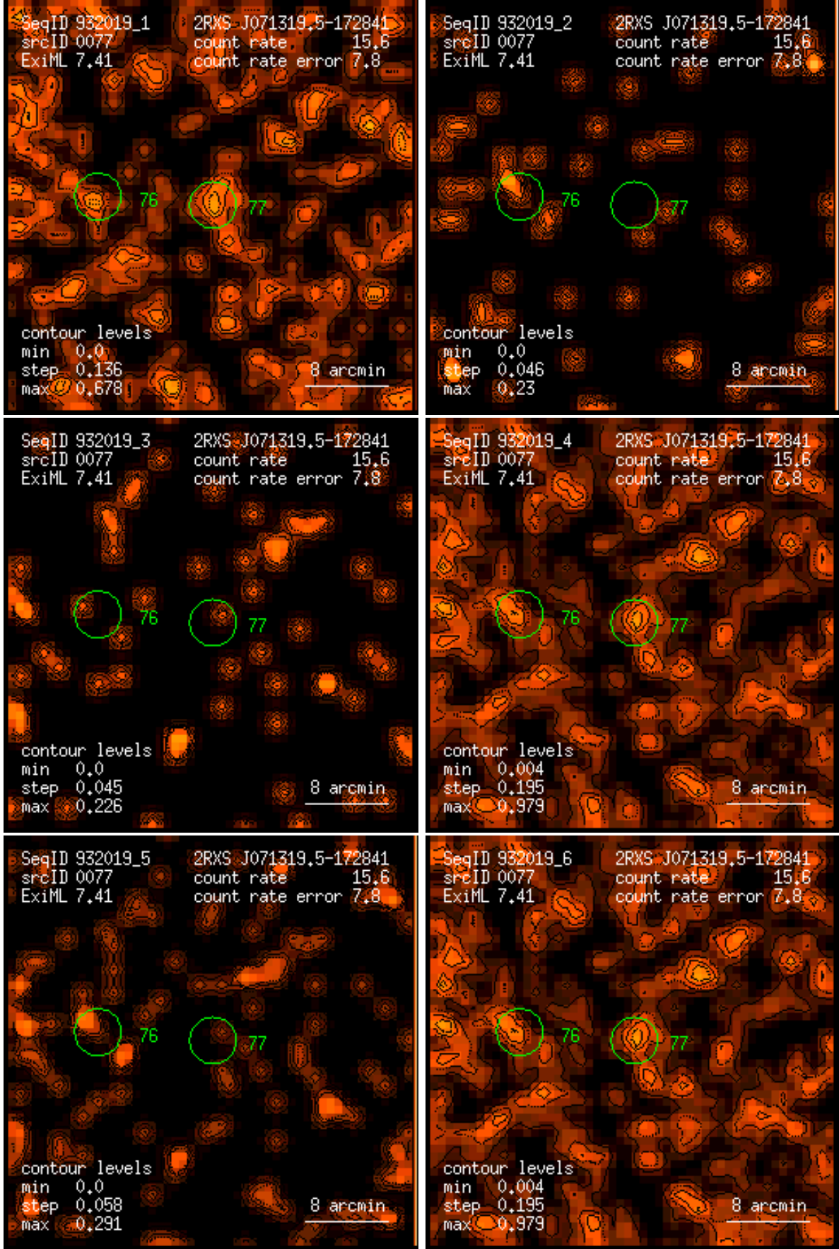
Figure 77: RASS 932019: detection 0077: band rate images, Gaussian filter: (1) PSPC channels 11 – 41, (2) 52 – 90, (3) 91 – 201, (4) 11 – 235, (5) 52 – 201, (6) 11 – 201. Broad band rates in counts/ks. Band rate contour levels in counts/ks/arcmin 2 .
