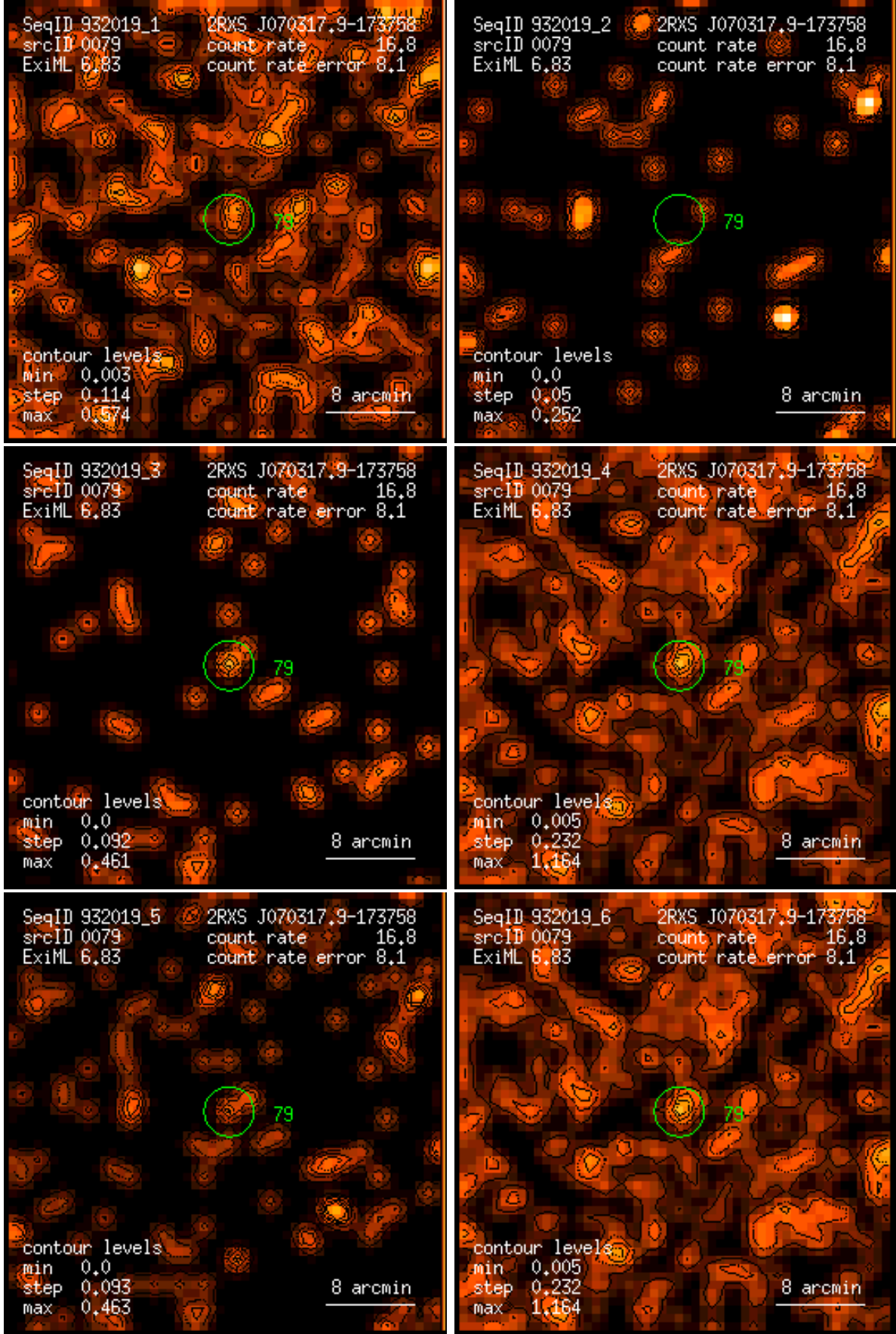
Figure 79: RASS 932019: detection 0079: band rate images, Gaussian filter: (1) PSPC channels 11 – 41, (2) 52 – 90, (3) 91 – 201, (4) 11 – 235, (5) 52 – 201, (6) 11 – 201. Broad band rates in counts/ks. Band rate contour levels in counts/ks/arcmin 2 .
