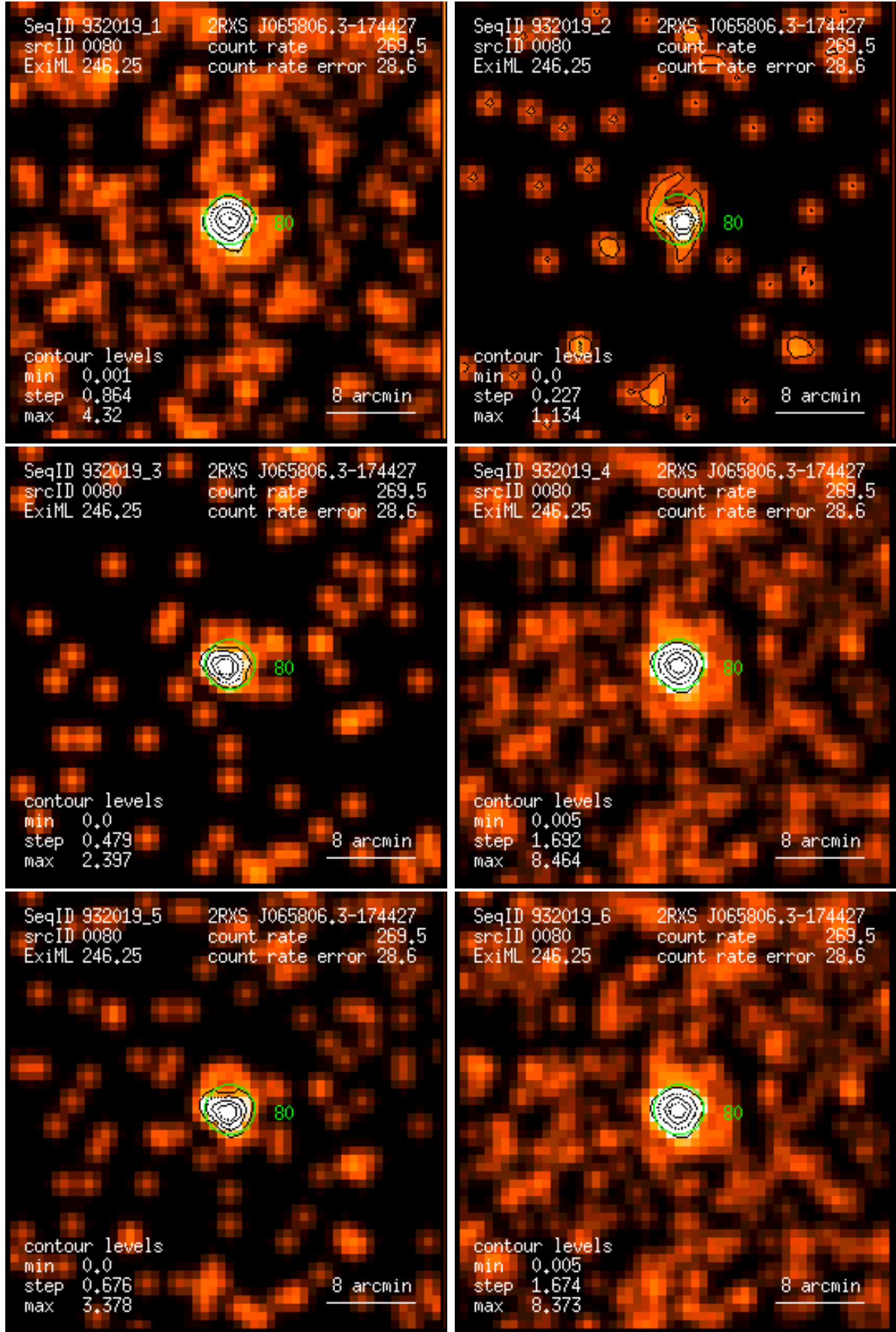
Figure 80: RASS 932019: detection 0080: band rate images, Gaussian filter: (1) PSPC channels 11 – 41, (2) 52 – 90, (3) 91 – 201, (4) 11 – 235, (5) 52 – 201, (6) 11 – 201. Broad band rates in counts/ks. Band rate contour levels in counts/ks/arcmin 2 .
