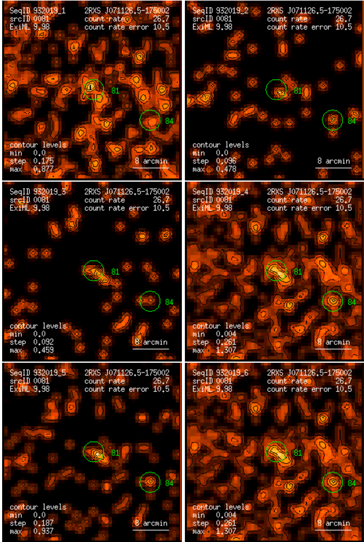
Figure 81: RASS 932019: detection 0081: band rate images, Gaussian filter: (1) PSPC channels 11 – 41, (2) 52 – 90, (3) 91 – 201, (4) 11 – 235, (5) 52 – 201, (6) 11 – 201. Broad band rates in counts/ks. Band rate contour levels in counts/ks/arcmin 2 .
