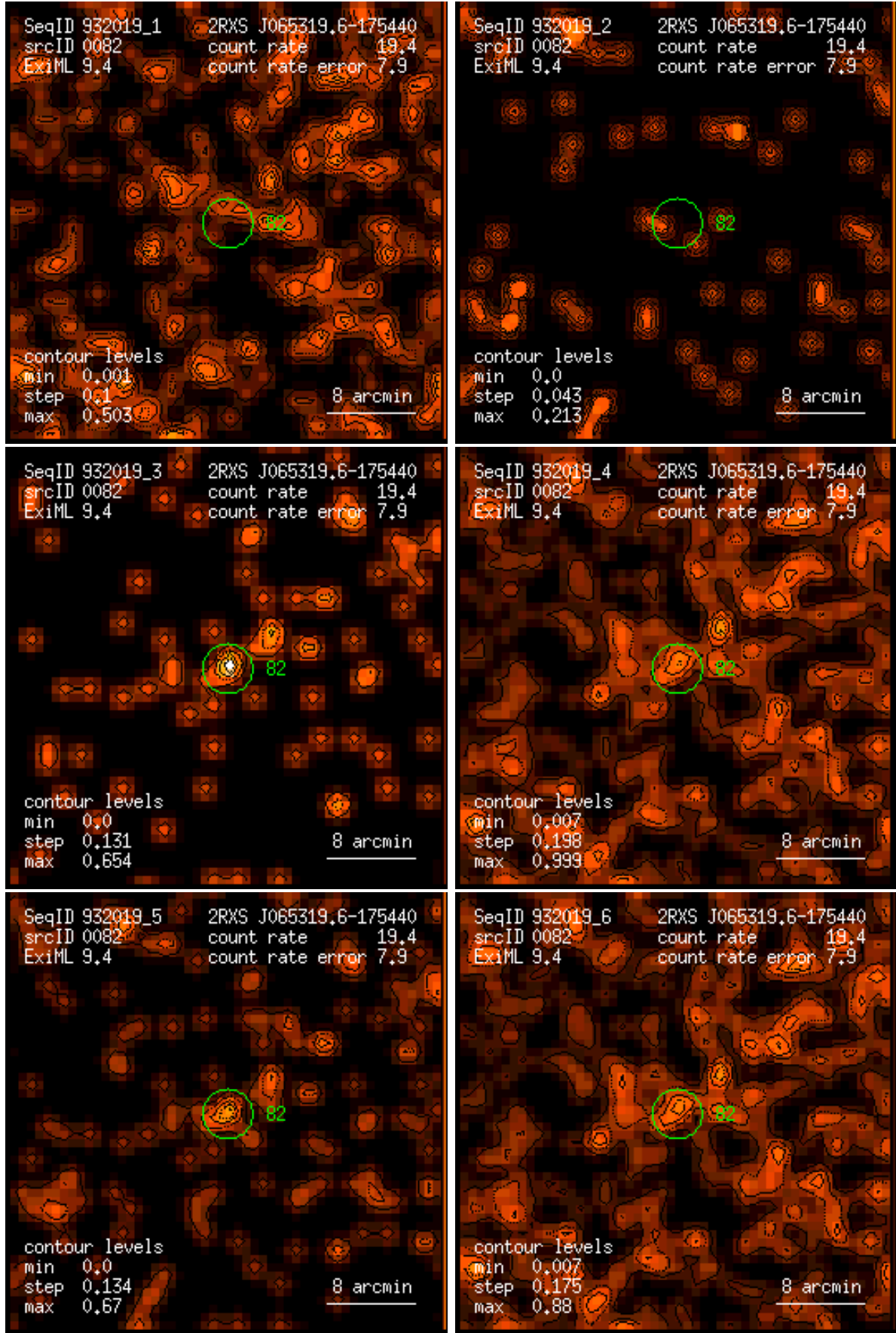
Figure 82: RASS 932019: detection 0082: band rate images, Gaussian filter: (1) PSPC channels 11 – 41, (2) 52 – 90, (3) 91 – 201, (4) 11 – 235, (5) 52 – 201, (6) 11 – 201. Broad band rates in counts/ks. Band rate contour levels in counts/ks/arcmin 2 .
