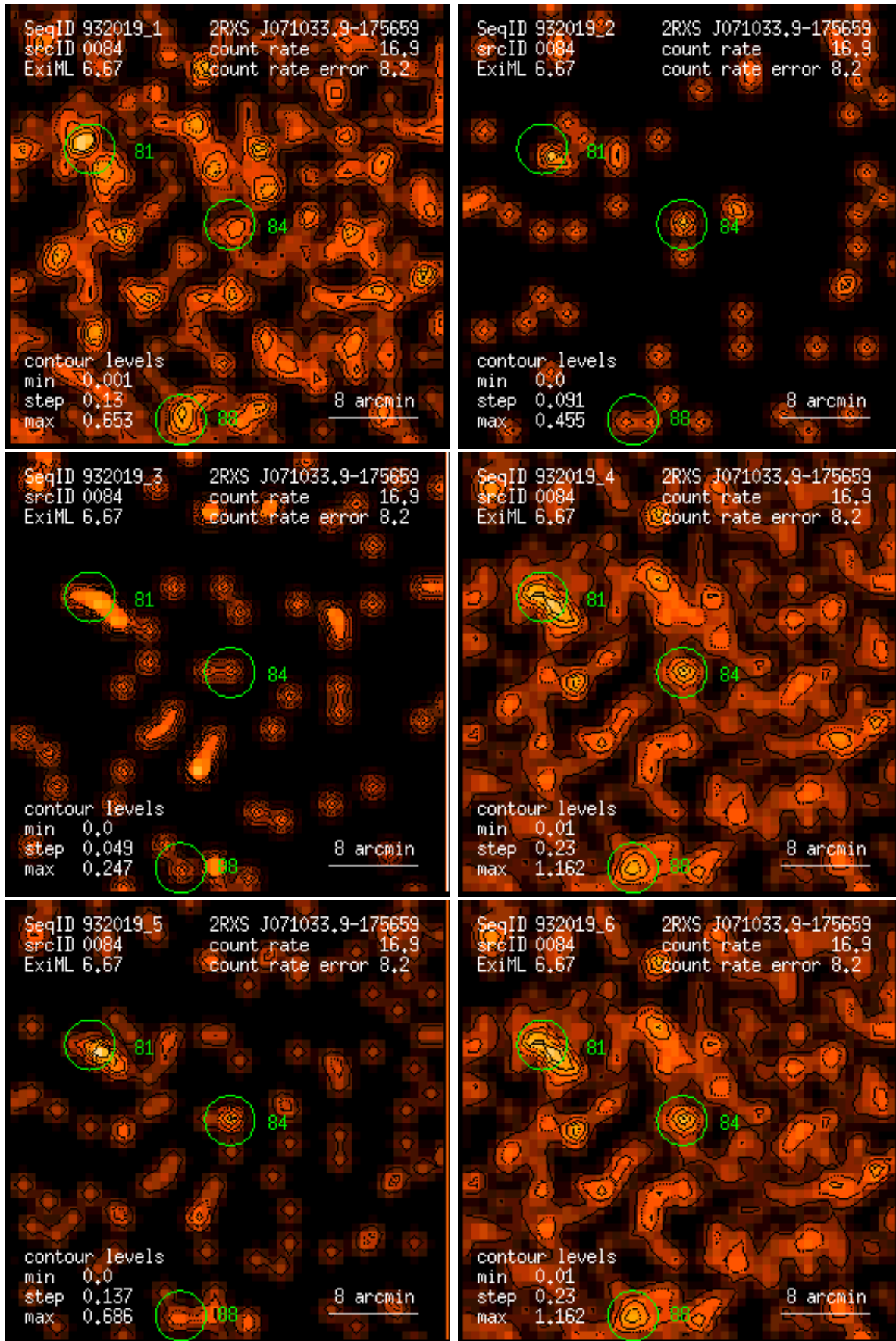
Figure 84: RASS 932019: detection 0084: band rate images, Gaussian filter: (1) PSPC channels 11 – 41, (2) 52 – 90, (3) 91 – 201, (4) 11 – 235, (5) 52 – 201, (6) 11 – 201. Broad band rates in counts/ks. Band rate contour levels in counts/ks/arcmin 2 .
