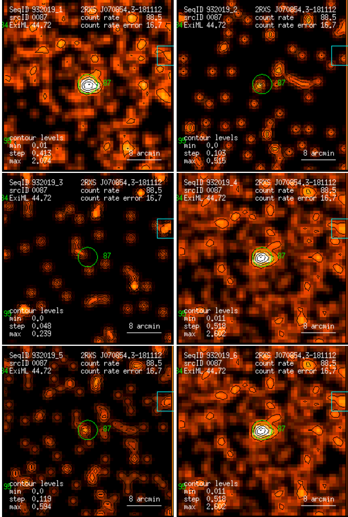
Figure 87: RASS 932019: detection 0087: band rate images, Gaussian filter: (1) PSPC channels 11 – 41, (2) 52 – 90, (3) 91 – 201, (4) 11 – 235, (5) 52 – 201, (6) 11 – 201. Broad band rates in counts/ks. Band rate contour levels in counts/ks/arcmin 2 .
