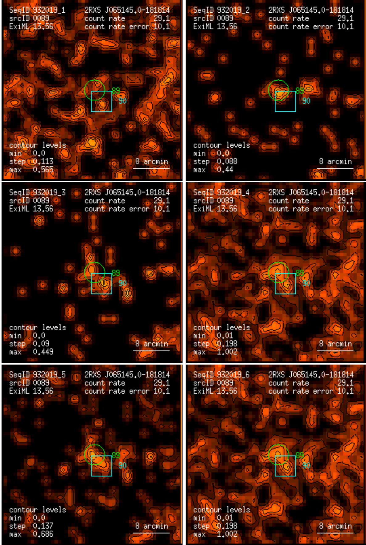
Figure 89: RASS 932019: detection 0089: band rate images, Gaussian filter: (1) PSPC channels 11 – 41, (2) 52 – 90, (3) 91 – 201, (4) 11 – 235, (5) 52 – 201, (6) 11 – 201. Broad band rates in counts/ks. Band rate contour levels in counts/ks/arcmin 2 .
