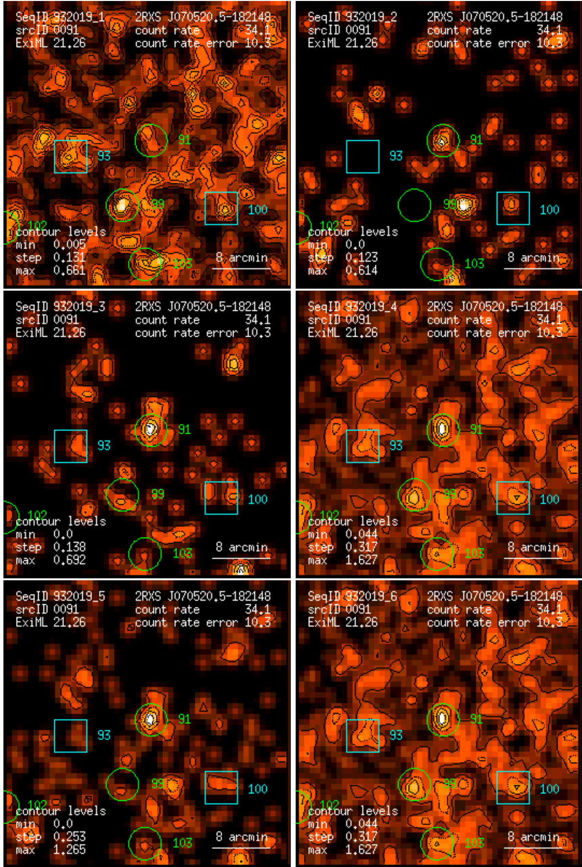
Figure 91: RASS 932019: detection 0091: band rate images, Gaussian filter: (1) PSPC channels 11 – 41, (2) 52 – 90, (3) 91 – 201, (4) 11 – 235, (5) 52 – 201, (6) 11 – 201. Broad band rates in counts/ks. Band rate contour levels in counts/ks/arcmin 2 .
