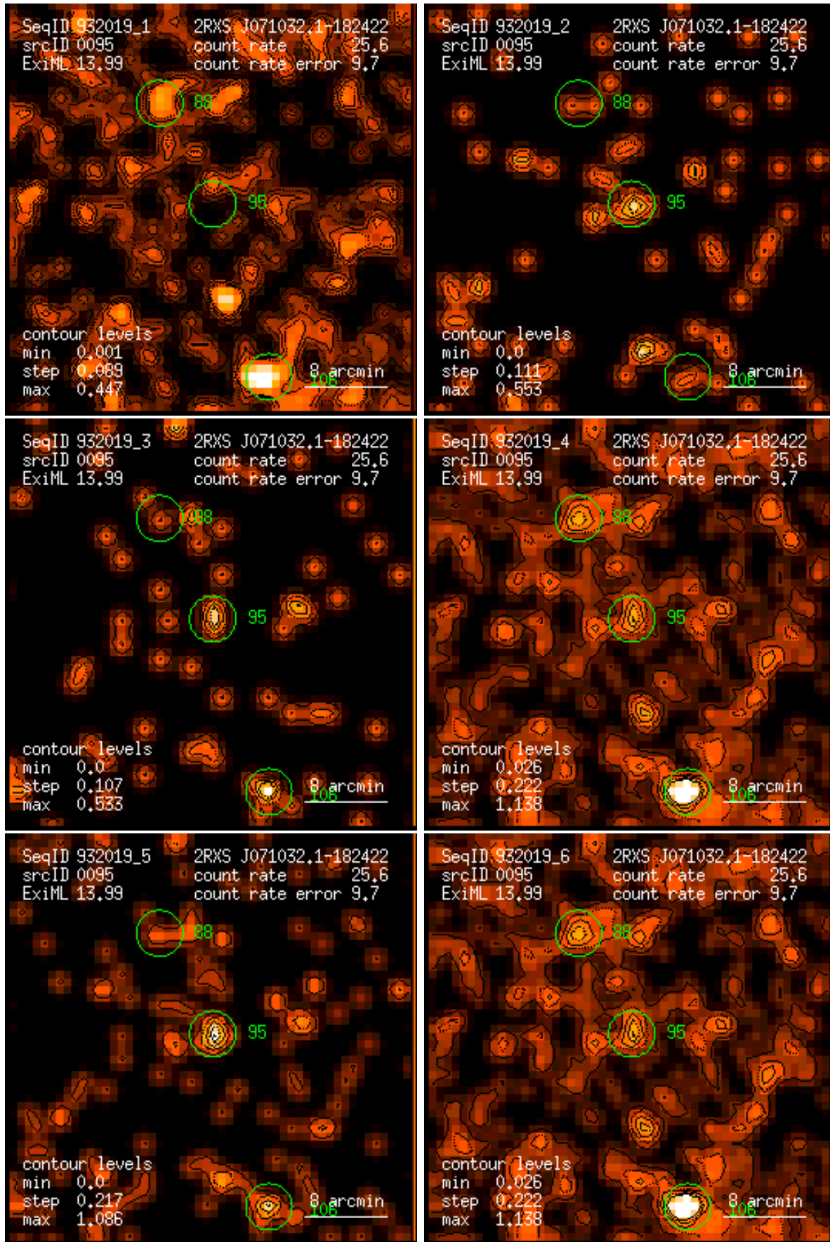
Figure 95: RASS 932019: detection 0095: band rate images, Gaussian filter: (1) PSPC channels 11 – 41, (2) 52 – 90, (3) 91 – 201, (4) 11 – 235, (5) 52 – 201, (6) 11 – 201. Broad band rates in counts/ks. Band rate contour levels in counts/ks/arcmin 2 .
