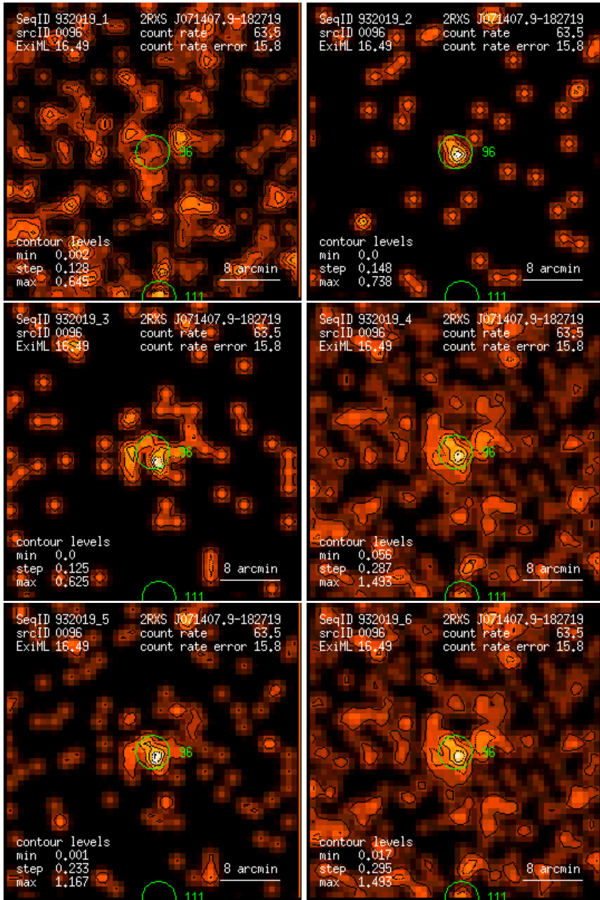
Figure 96: RASS 932019: detection 0096: band rate images, Gaussian filter: (1) PSPC channels 11 – 41, (2) 52 – 90, (3) 91 – 201, (4) 11 – 235, (5) 52 – 201, (6) 11 – 201. Broad band rates in counts/ks. Band rate contour levels in counts/ks/arcmin 2 .
