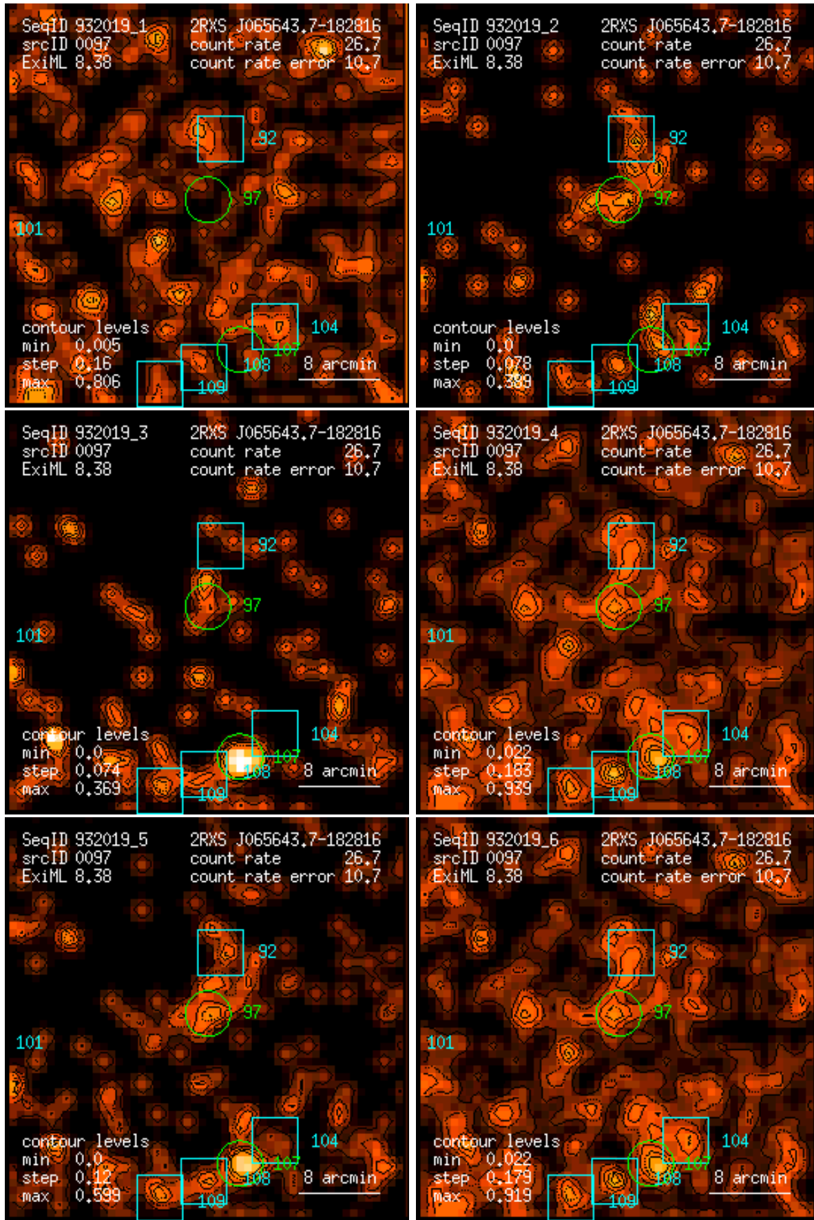
Figure 97: RASS 932019: detection 0097: band rate images, Gaussian filter: (1) PSPC channels 11 – 41, (2) 52 – 90, (3) 91 – 201, (4) 11 – 235, (5) 52 – 201, (6) 11 – 201. Broad band rates in counts/ks. Band rate contour levels in counts/ks/arcmin 2 .
