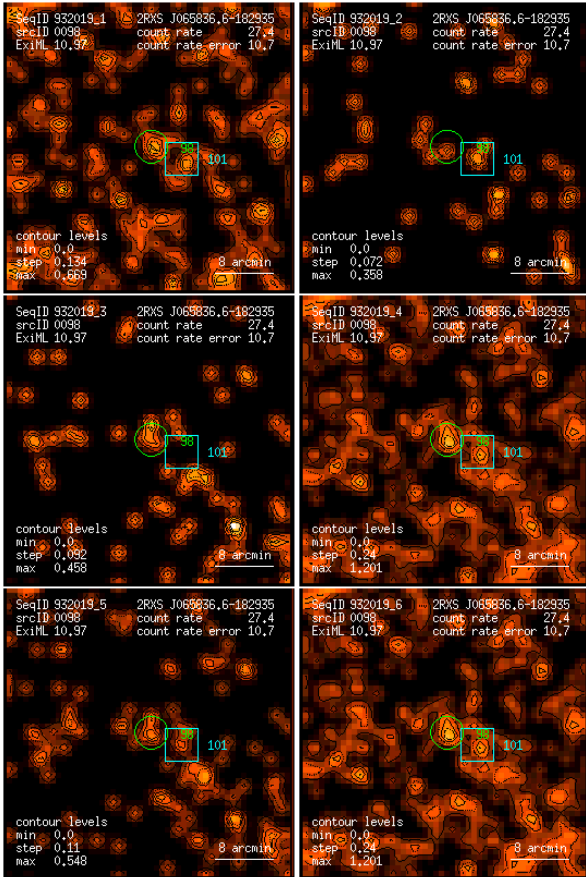
Figure 98: RASS 932019: detection 0098: band rate images, Gaussian filter: (1) PSPC channels 11 – 41, (2) 52 – 90, (3) 91 – 201, (4) 11 – 235, (5) 52 – 201, (6) 11 – 201. Broad band rates in counts/ks. Band rate contour levels in counts/ks/arcmin 2 .
