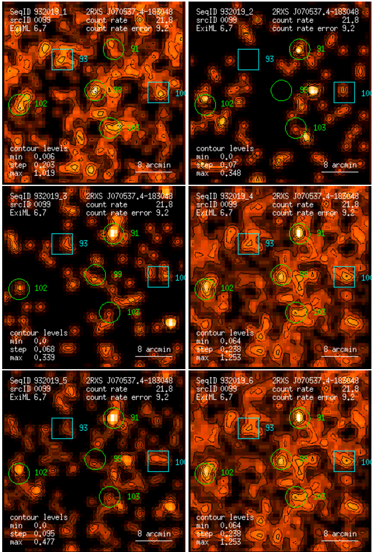
Figure 99: RASS 932019: detection 0099: band rate images, Gaussian filter: (1) PSPC channels 11 – 41, (2) 52 – 90, (3) 91 – 201, (4) 11 – 235, (5) 52 – 201, (6) 11 – 201. Broad band rates in counts/ks. Band rate contour levels in counts/ks/arcmin 2 .
