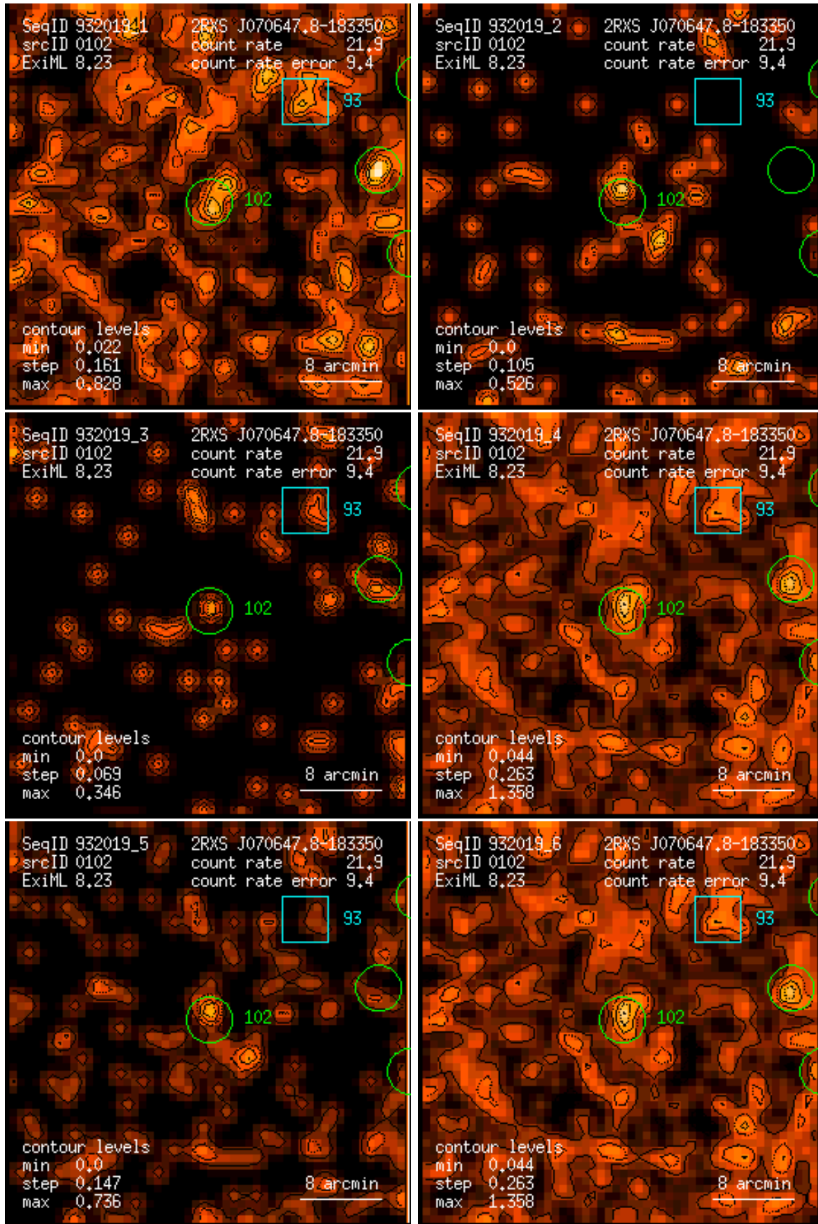
Figure 102: RASS 932019: detection 0102: band rate images, Gaussian filter: (1) PSPC channels 11 – 41, (2) 52 – 90, (3) 91 – 201, (4) 11 – 235, (5) 52 – 201, (6) 11 – 201. Broad band rates in counts/ks. Band rate contour levels in counts/ks/arcmin 2 .
