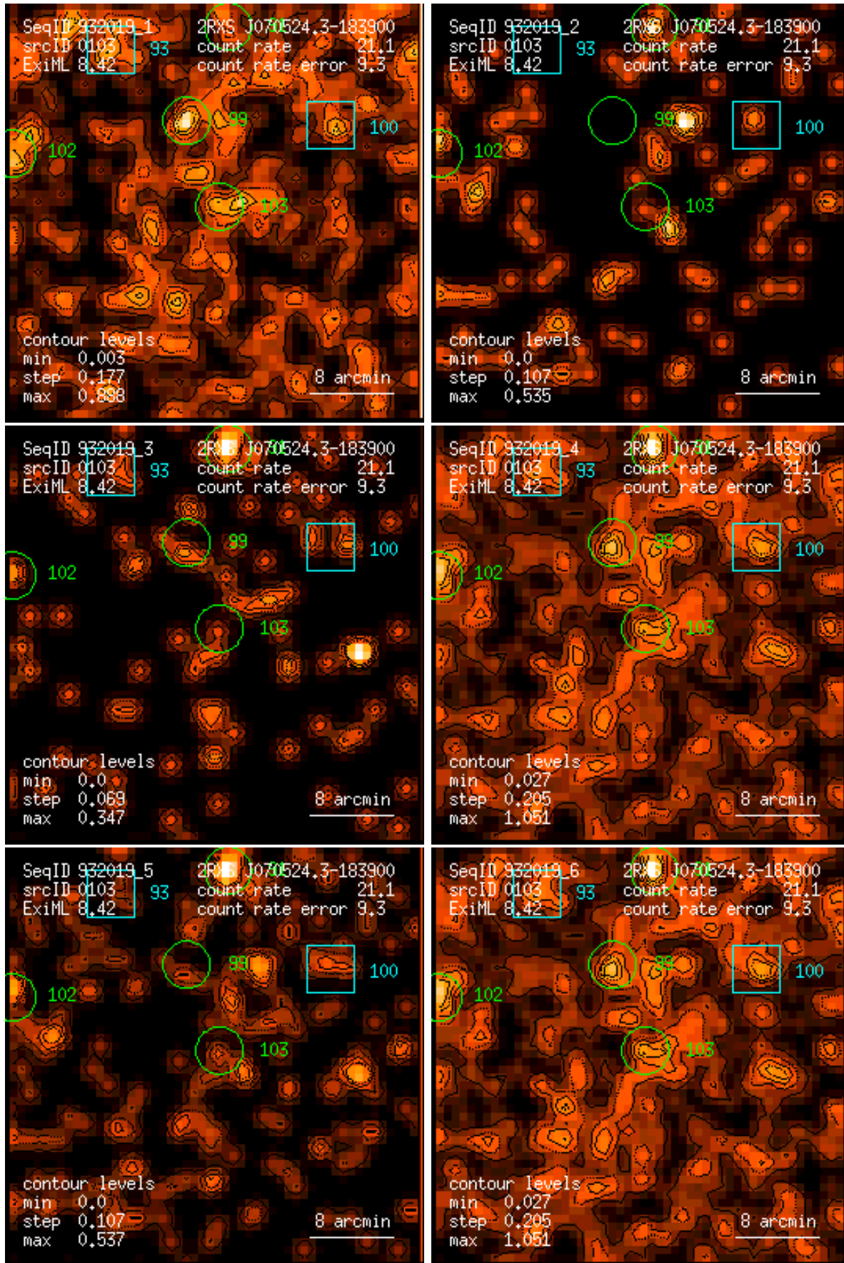
Figure 103: RASS 932019: detection 0103: band rate images, Gaussian filter: (1) PSPC channels 11 – 41, (2) 52 – 90, (3) 91 – 201, (4) 11 – 235, (5) 52 – 201, (6) 11 – 201. Broad band rates in counts/ks. Band rate contour levels in counts/ks/arcmin 2 .
