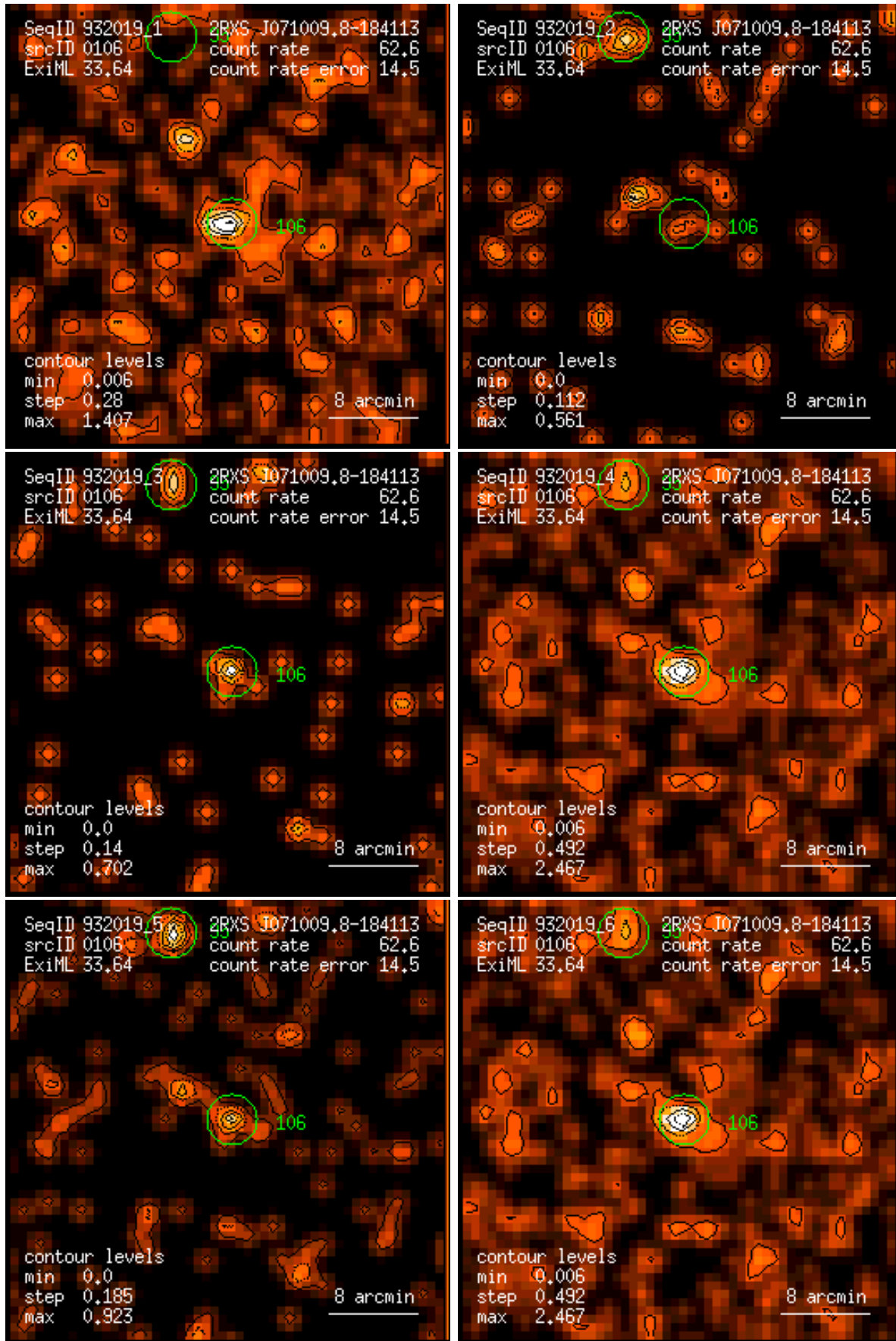
Figure 106: RASS 932019: detection 0106: band rate images, Gaussian filter: (1) PSPC channels 11 – 41, (2) 52 – 90, (3) 91 – 201, (4) 11 – 235, (5) 52 – 201, (6) 11 – 201. Broad band rates in counts/ks. Band rate contour levels in counts/ks/arcmin 2 .
