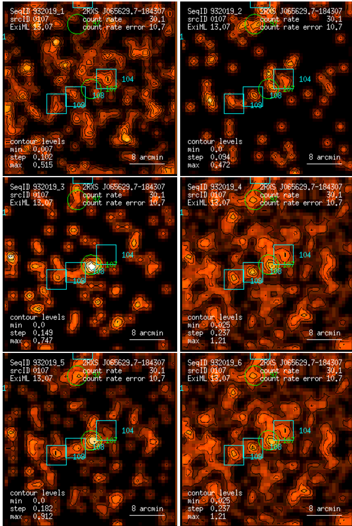
Figure 107: RASS 932019: detection 0107: band rate images, Gaussian filter: (1) PSPC channels 11 – 41, (2) 52 – 90, (3) 91 – 201, (4) 11 – 235, (5) 52 – 201, (6) 11 – 201. Broad band rates in counts/ks. Band rate contour levels in counts/ks/arcmin 2 .
