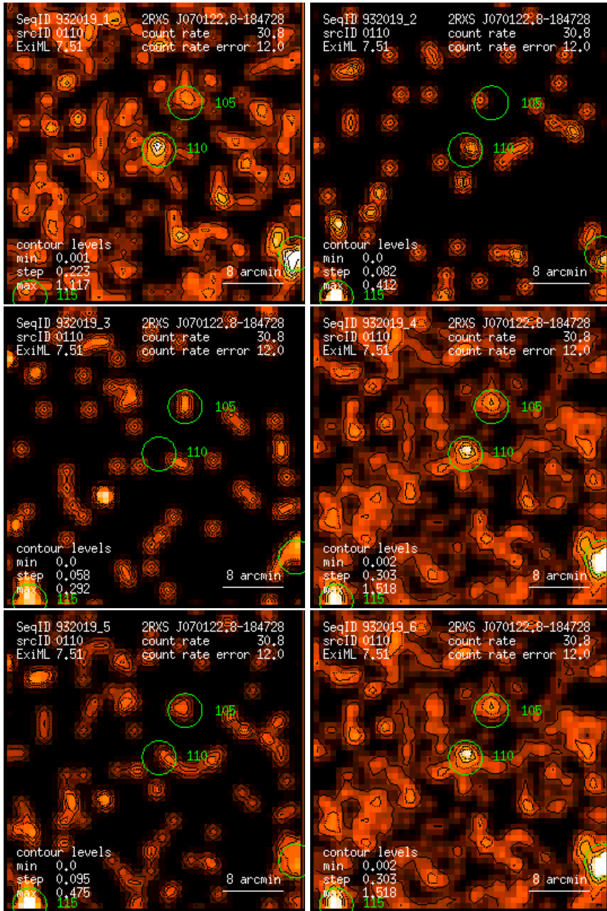
Figure 110: RASS 932019: detection 0110: band rate images, Gaussian filter: (1) PSPC channels 11 – 41, (2) 52 – 90, (3) 91 – 201, (4) 11 – 235, (5) 52 – 201, (6) 11 – 201. Broad band rates in counts/ks. Band rate contour levels in counts/ks/arcmin 2 .
