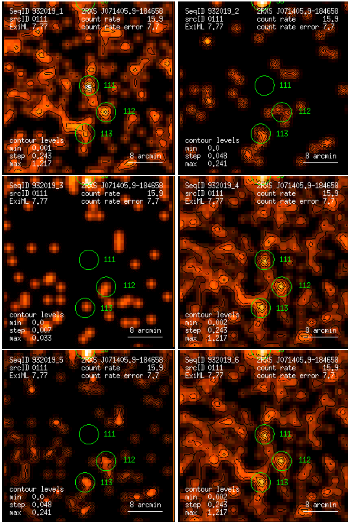
Figure 111: RASS 932019: detection 0111: band rate images, Gaussian filter: (1) PSPC channels 11 – 41, (2) 52 – 90, (3) 91 – 201, (4) 11 – 235, (5) 52 – 201, (6) 11 – 201. Broad band rates in counts/ks. Band rate contour levels in counts/ks/arcmin 2 .
