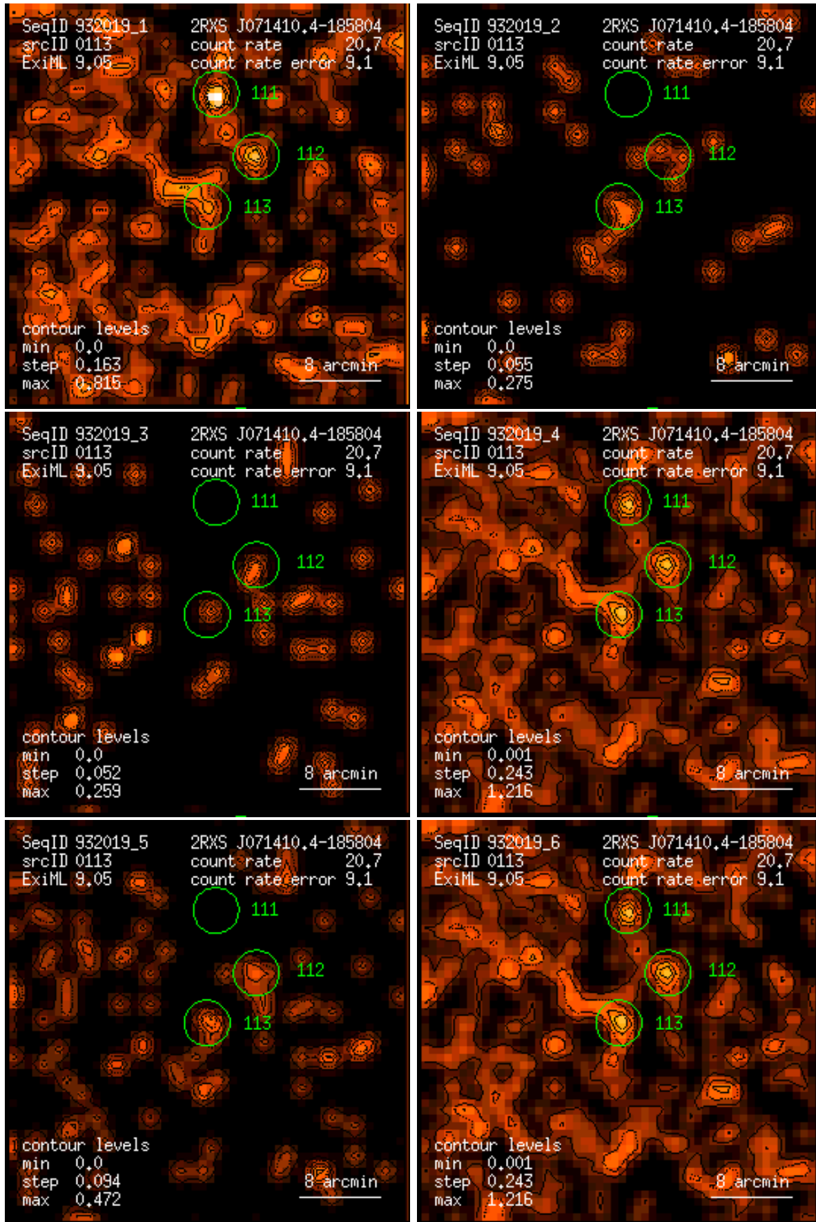
Figure 113: RASS 932019: detection 0113: band rate images, Gaussian filter: (1) PSPC channels 11 – 41, (2) 52 – 90, (3) 91 – 201, (4) 11 – 235, (5) 52 – 201, (6) 11 – 201. Broad band rates in counts/ks. Band rate contour levels in counts/ks/arcmin 2 .
