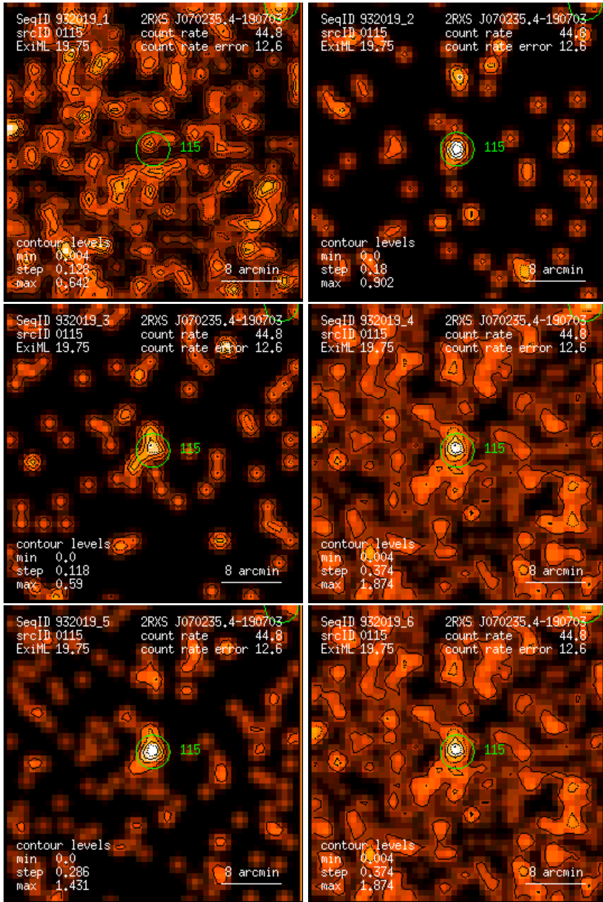
Figure 115: RASS 932019: detection 0115: band rate images, Gaussian filter: (1) PSPC channels 11 – 41, (2) 52 – 90, (3) 91 – 201, (4) 11 – 235, (5) 52 – 201, (6) 11 – 201. Broad band rates in counts/ks. Band rate contour levels in counts/ks/arcmin 2 .
