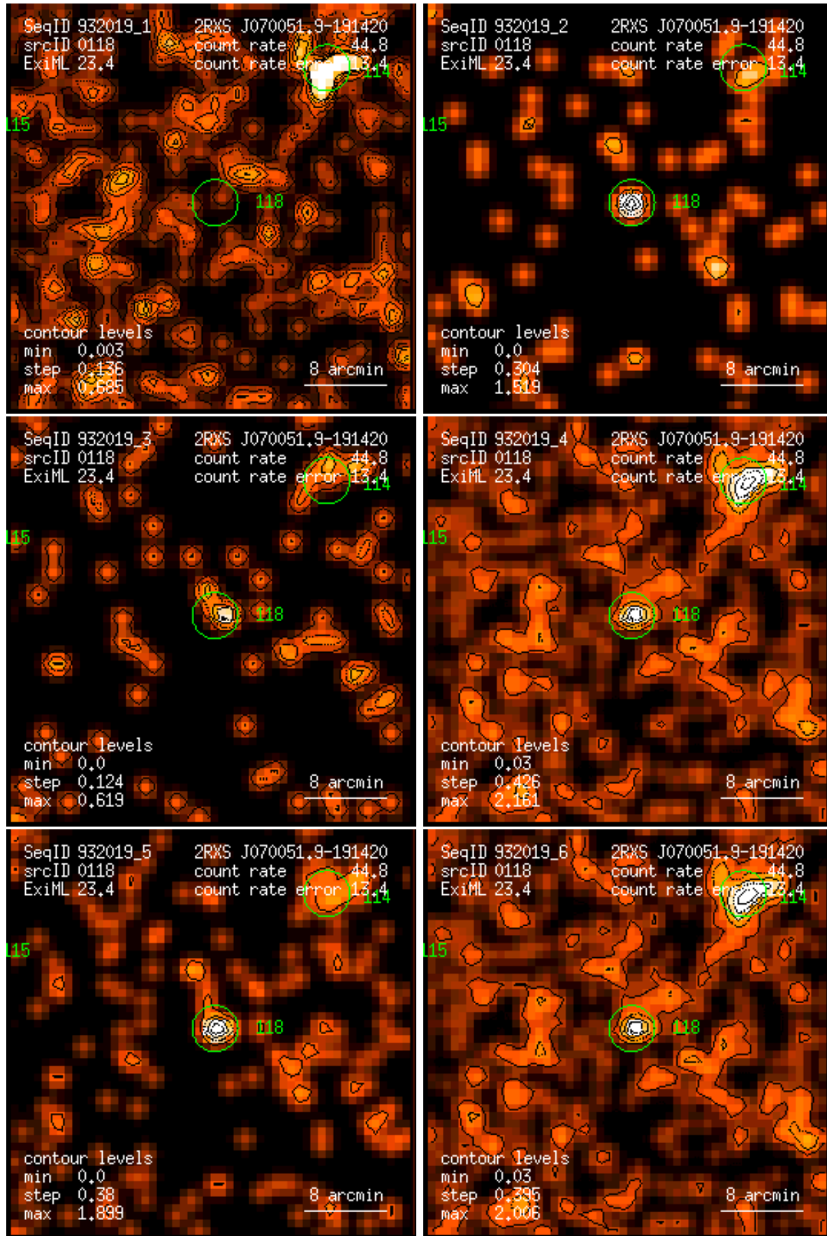
Figure 118: RASS 932019: detection 0118: band rate images, Gaussian filter: (1) PSPC channels 11 – 41, (2) 52 – 90, (3) 91 – 201, (4) 11 – 235, (5) 52 – 201, (6) 11 – 201. Broad band rates in counts/ks. Band rate contour levels in counts/ks/arcmin 2 .
