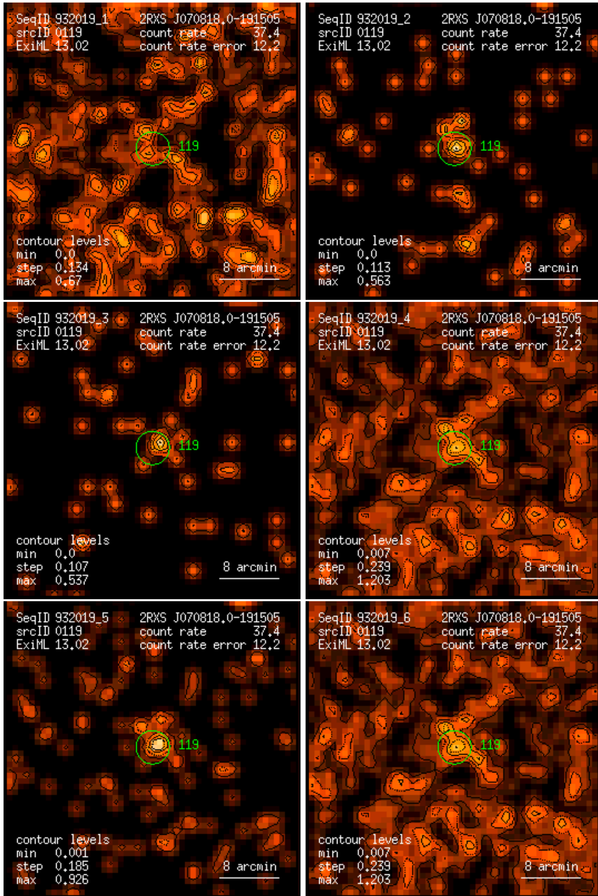
Figure 119: RASS 932019: detection 0119: band rate images, Gaussian filter: (1) PSPC channels 11 – 41, (2) 52 – 90, (3) 91 – 201, (4) 11 – 235, (5) 52 – 201, (6) 11 – 201. Broad band rates in counts/ks. Band rate contour levels in counts/ks/arcmin 2 .
