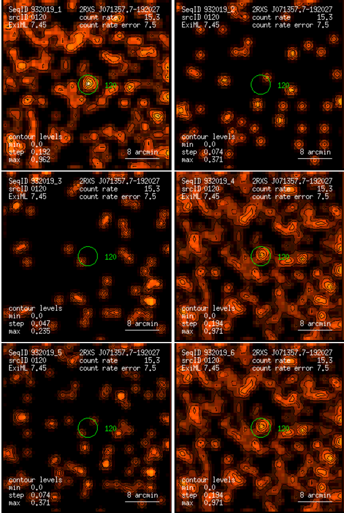
Figure 120: RASS 932019: detection 0120: band rate images, Gaussian filter: (1) PSPC channels 11 – 41, (2) 52 – 90, (3) 91 – 201, (4) 11 – 235, (5) 52 – 201, (6) 11 – 201. Broad band rates in counts/ks. Band rate contour levels in counts/ks/arcmin 2 .
