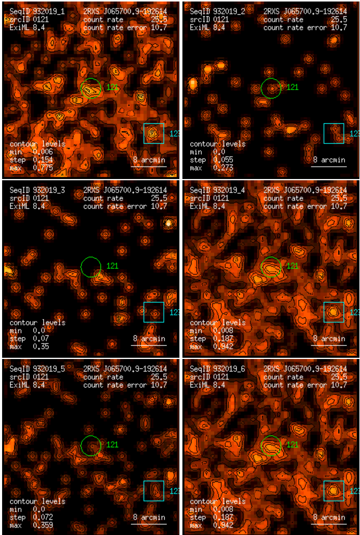
Figure 121: RASS 932019: detection 0121: band rate images, Gaussian filter: (1) PSPC channels 11 – 41, (2) 52 – 90, (3) 91 – 201, (4) 11 – 235, (5) 52 – 201, (6) 11 – 201. Broad band rates in counts/ks. Band rate contour levels in counts/ks/arcmin 2 .
